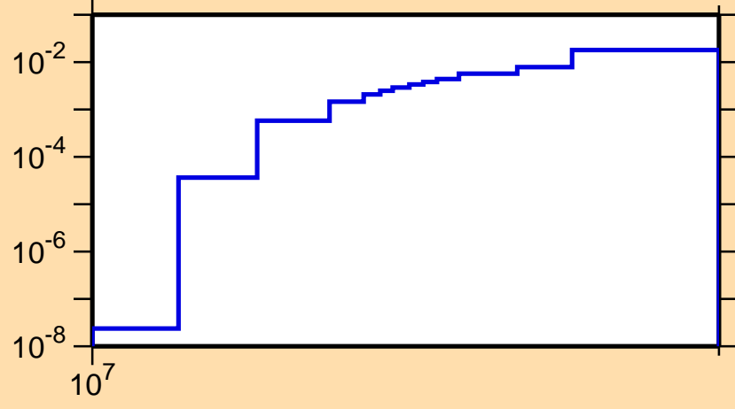
\sigma vs. E for ^{13}\text{N}(n,n\alpha)
