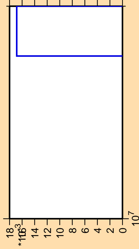
\Delta\sigma/\sigma vs. E for ^{13}\text{N}(n,\text{nd})
