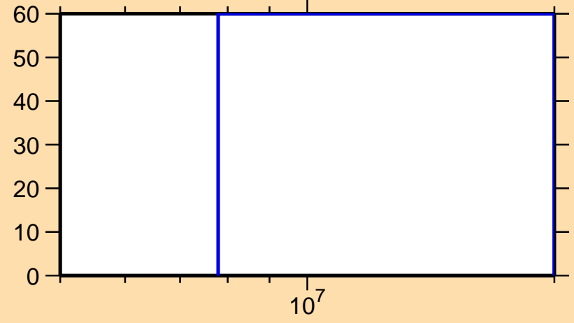
\Delta\sigma/\sigma vs. E for ^{13}\text{N}(n,ncont.)
