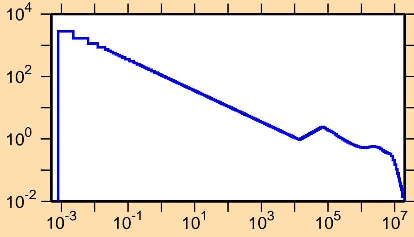
\sigma vs. E for ^{13}\text{N}(n,p)
