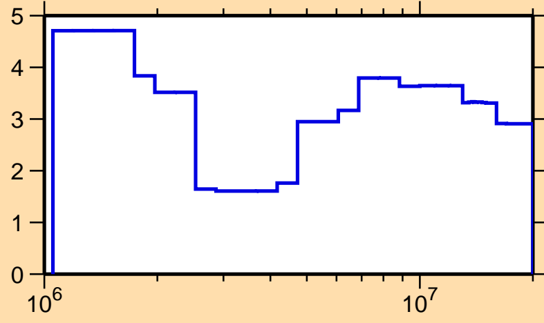
\Delta\sigma/\sigma vs. E for ^{13}\text{N}(n,\text{el.})
