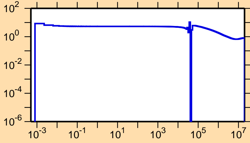
\sigma vs. E for ^{13}\text{N}(n,\text{el.})
