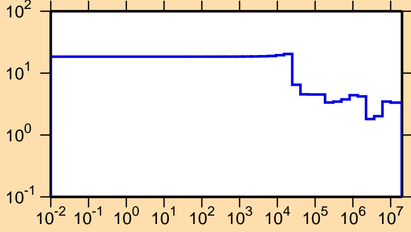
\Delta\sigma/\sigma vs. E for ^{13}\text{N}(n,\text{el.})
