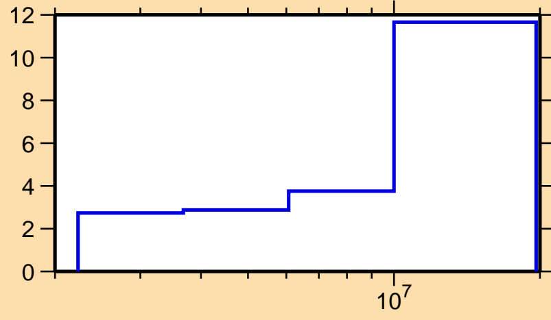
\Delta\sigma/\sigma vs. E for ^{13}\text{N}(n,\text{inel.})
