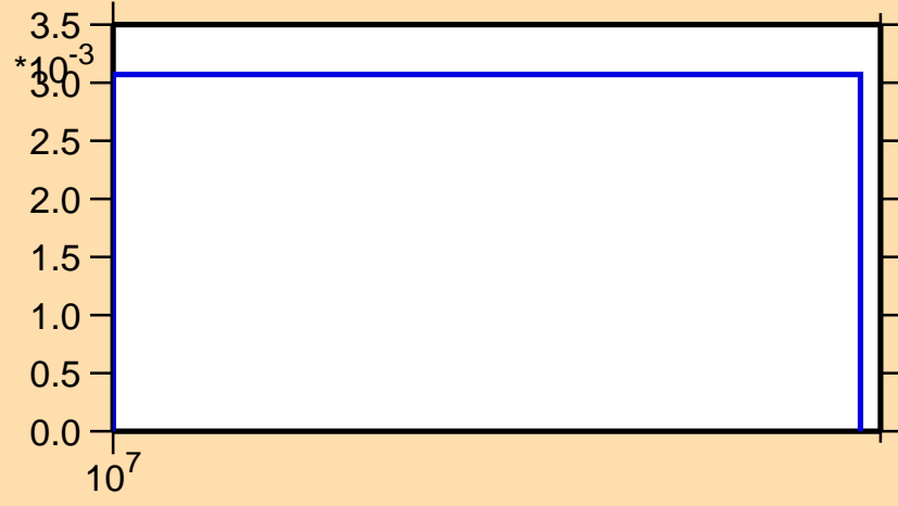
\sigma vs. E for ^{13}\text{N}(n,n\alpha)
