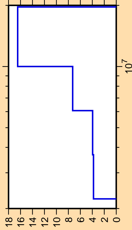
\Delta\sigma/\sigma vs. E for ^{13}\text{N}(n,p)
