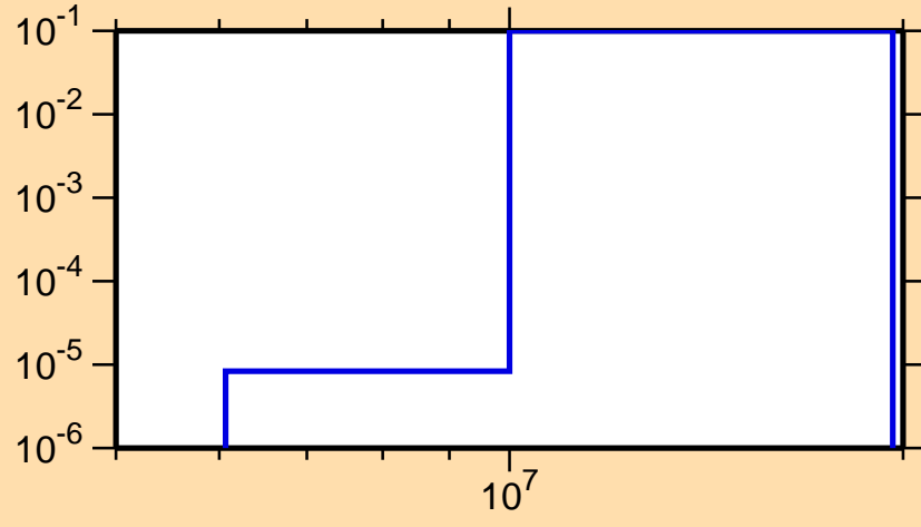
\sigma vs. E for ^{13}\text{N}(\text{mt117})
