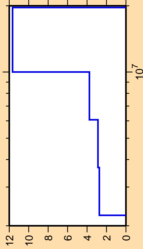
\Delta\sigma/\sigma vs. E for ^{13}\text{N}(n,\text{inel.})
