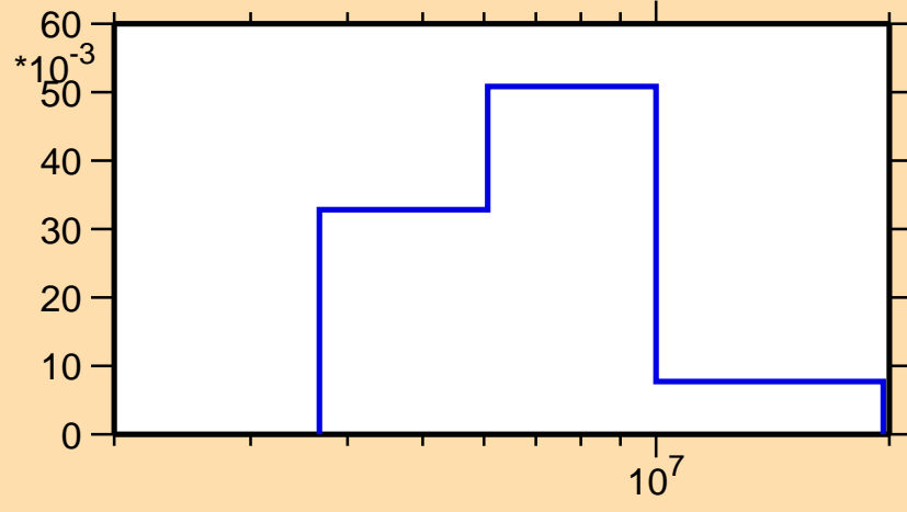
\sigma vs. E for ^{13}\text{N}(n,n_3)
