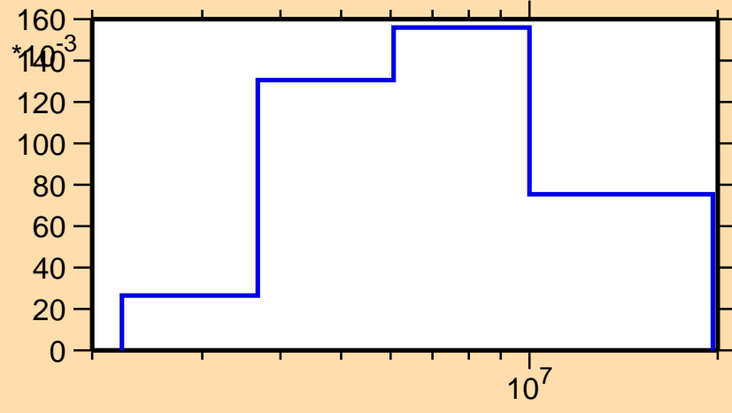
\sigma vs. E for ^{13}\text{N}(n,\text{inel.})
