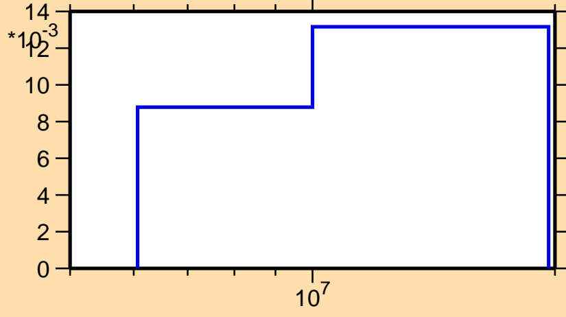
\sigma vs. E for ^{13}\text{N}(n,n_4)
