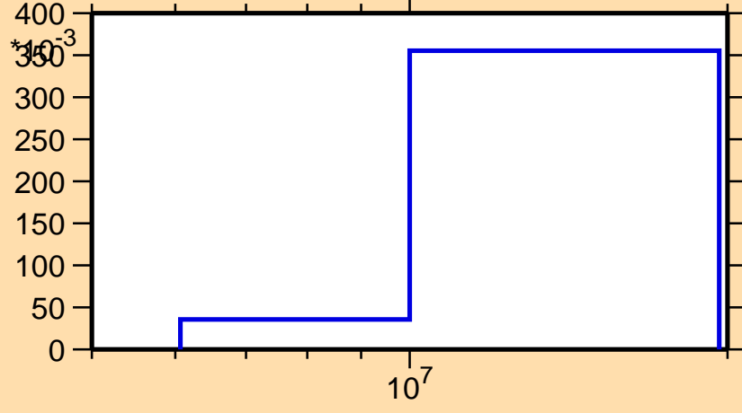
\sigma vs. E for ^{13}\text{N}(n,np)
