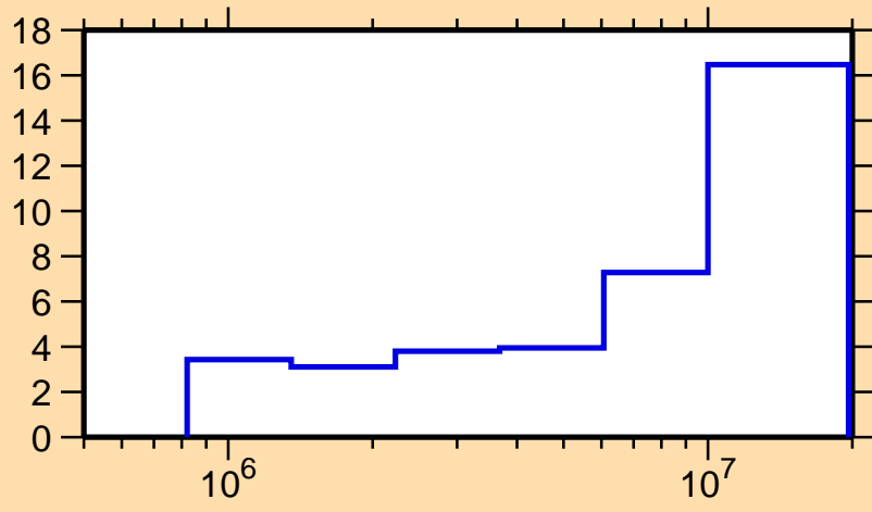
\Delta\sigma/\sigma vs. E for ^{13}\text{N}(n,p)
