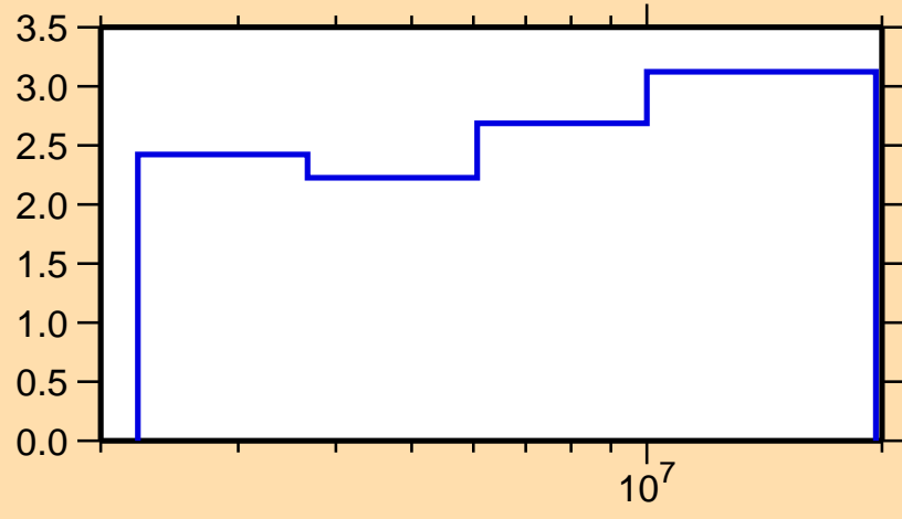
\Delta\sigma/\sigma vs. E for ^{13}\text{N}(n,\text{nonel.})
