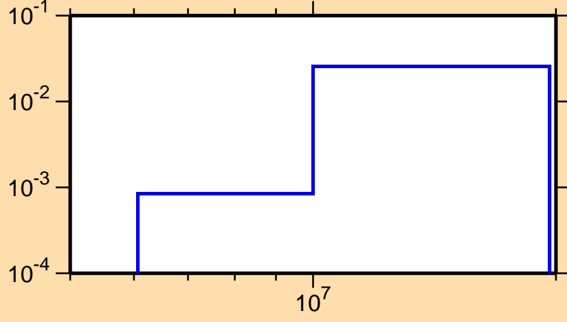
\sigma vs. E for ^{13}\text{N}(n,n\text{cont.})
