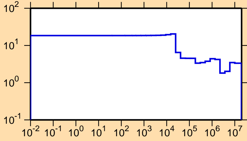
\Delta\sigma/\sigma vs. E for ^{13}\text{N}(n,el.)
