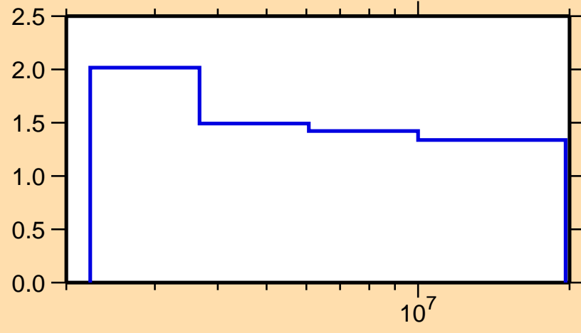
\Delta\sigma/\sigma vs. E for ^{13}\text{N}(n,\text{tot.})
