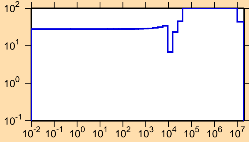
\Delta\sigma/\sigma vs. E for ^{13}\text{N}(n,\gamma)
