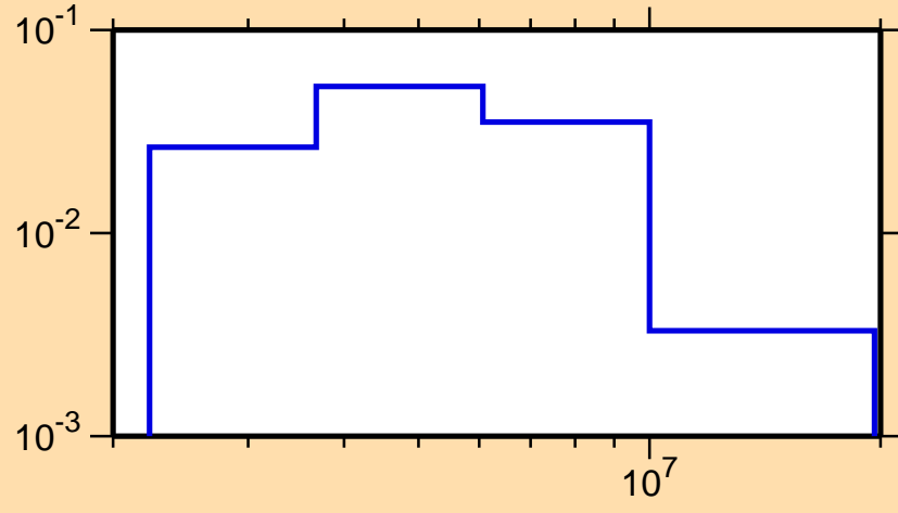
\sigma vs. E for ^{13}\text{N}(n,n_1)
