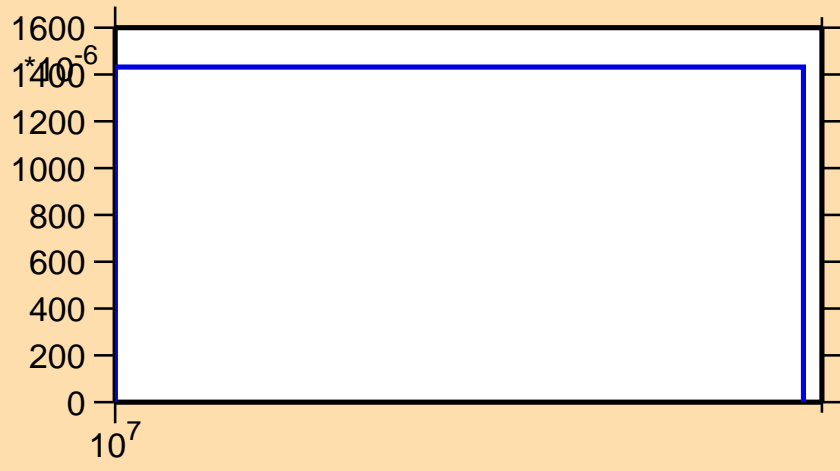
\sigma vs. E for ^{13}\text{N} (mt 45)
