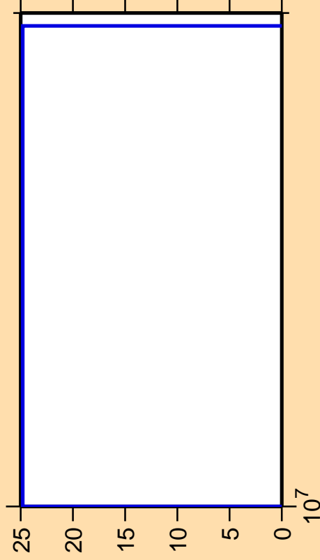
\Delta\sigma/\sigma vs. E for ^{13}\text{N} (mt 45)
