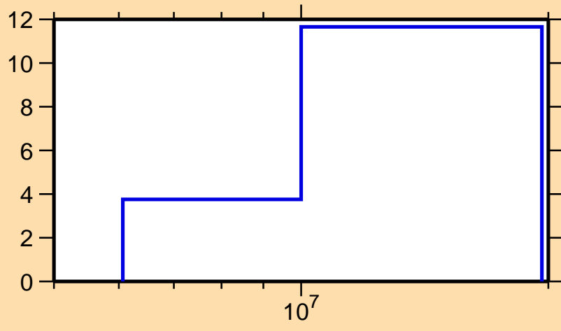
\Delta\sigma/\sigma vs. E for ^{13}\text{N}(n,\text{inel.})
