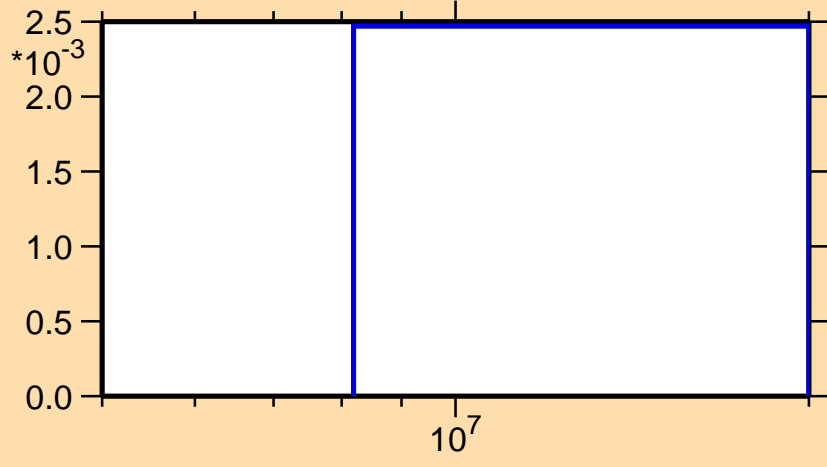
\sigma vs. E for ^{13}\text{N}(n,\alpha)
