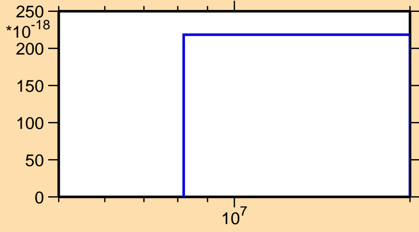
\sigma vs. E for ^{13}\text{N}(n,\text{nd})
