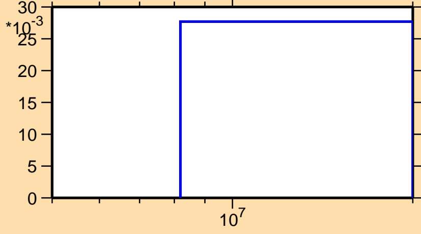
\sigma vs. E for ^{13}\text{N}(n,p\alpha)
