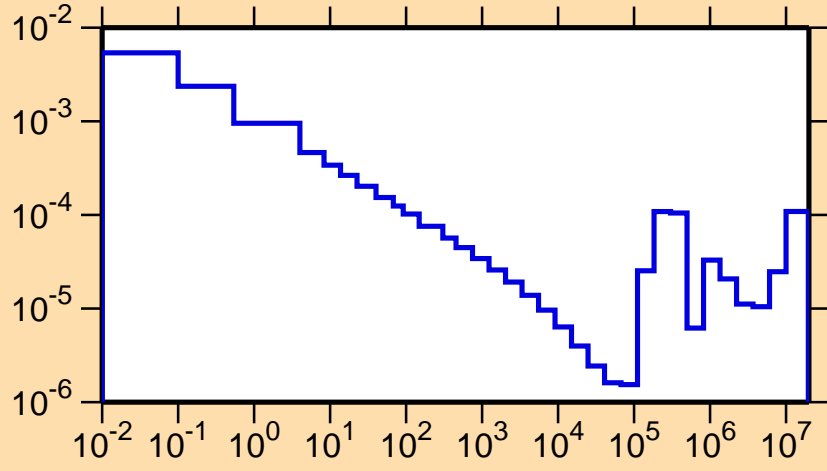
\sigma vs. E for ^{16}\text{N}(n,\gamma)
