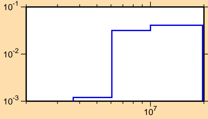
\sigma vs. E for ^{16}\text{N}(n,t)
