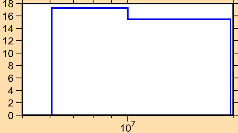
\Delta\sigma/\sigma vs. E for ^{16}\text{N}(n,p)
