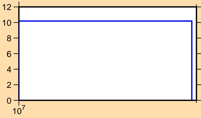
\Delta\sigma/\sigma vs. E for ^{17}\text{N}(n,p)
