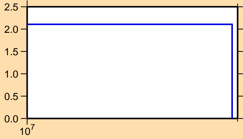
\Delta\sigma/\sigma vs. E for ^{17}\text{N}(n,el.)
