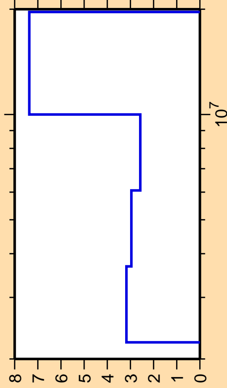
\Delta\sigma/\sigma vs. E for ^{17}\text{N}(n,n_4)
