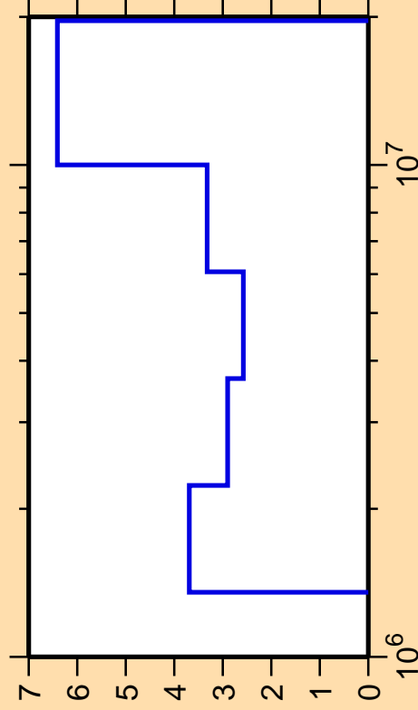
\Delta\sigma/\sigma vs. E for ^{17}\text{N}(n,n_2)
