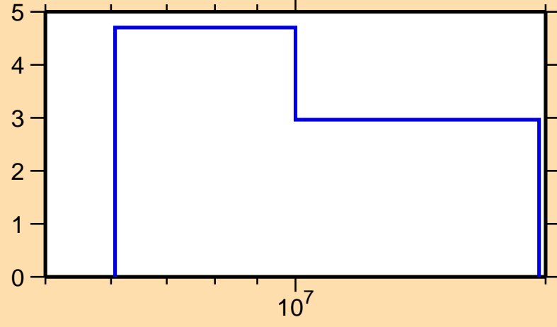
\Delta\sigma/\sigma vs. E for ^{17}\text{N}(n,2n)
