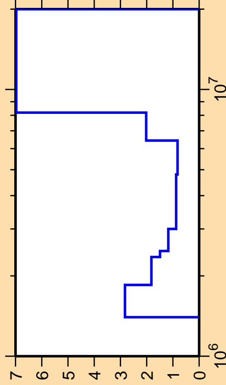
\Delta\sigma/\sigma vs. E for ^{17}\text{N}(n,n_1)
