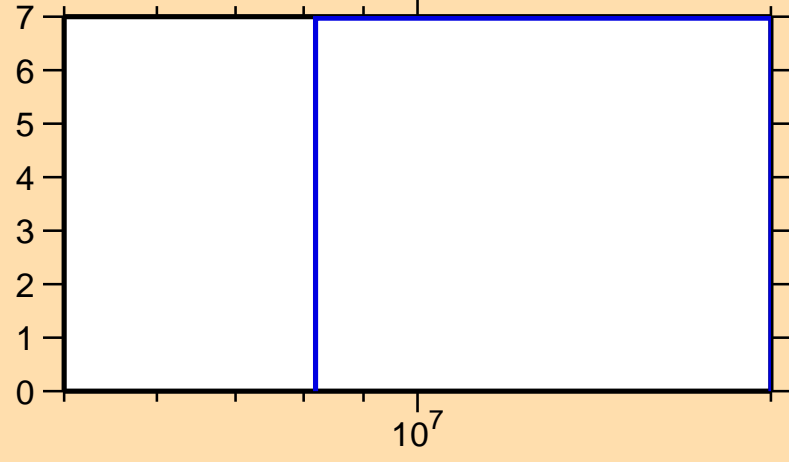
\Delta\sigma/\sigma vs. E for ^{17}\text{N}(n, n_1)
