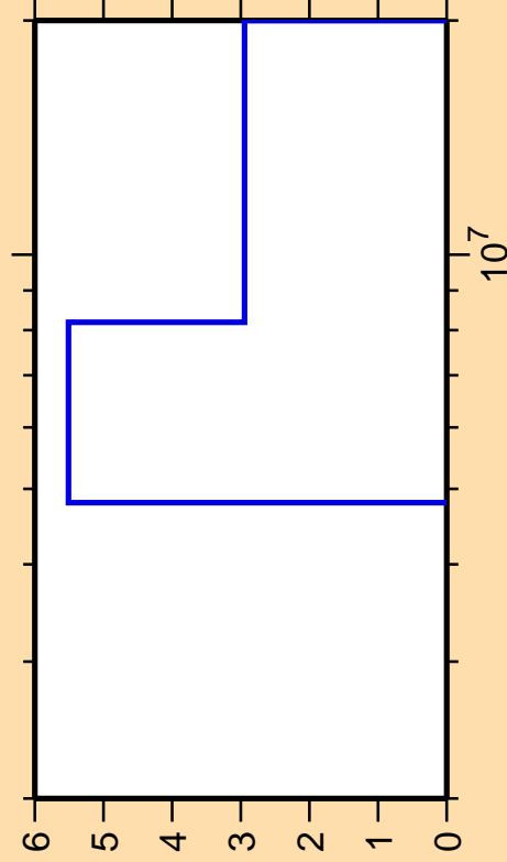
\Delta\sigma/\sigma vs. E for ^{17}\text{N}(n,2n)
