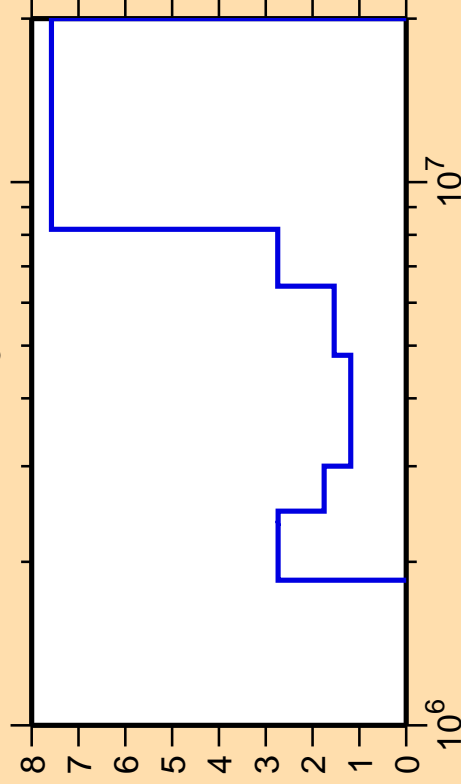
\Delta\sigma/\sigma vs. E for ^{17}\text{N}(n,n_3)
