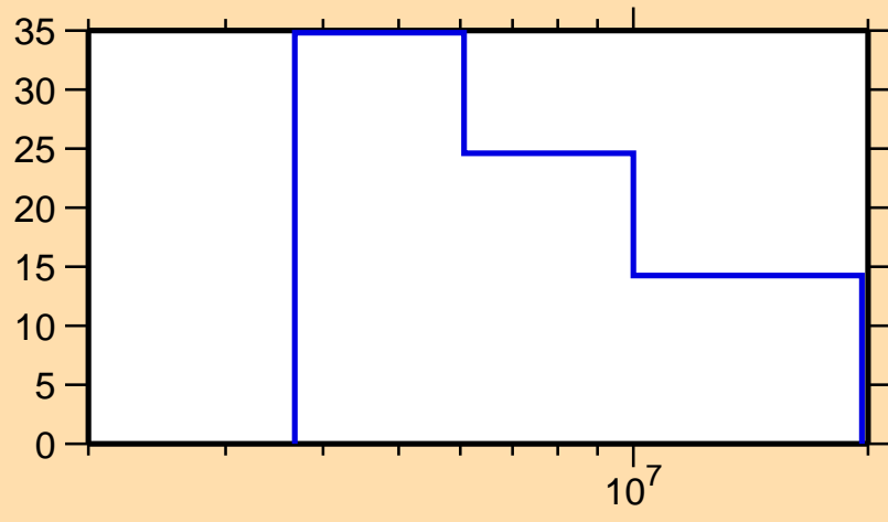
\Delta\sigma/\sigma vs. E for ^{21}\text{Na}(n,ncont.)
