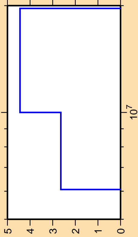
\Delta\sigma/\sigma vs. E for ^{21}\text{Na}(n,n\alpha)
