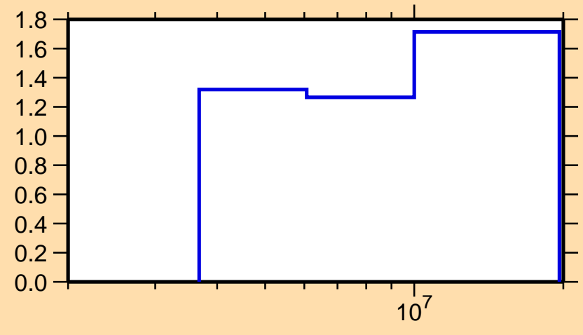
\Delta\sigma/\sigma vs. E for ^{21}\text{Na}(n,n\text{nonel.})
