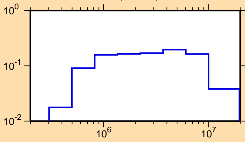
\sigma vs. E for ^{21}\text{Na}(n,\text{inel.})
