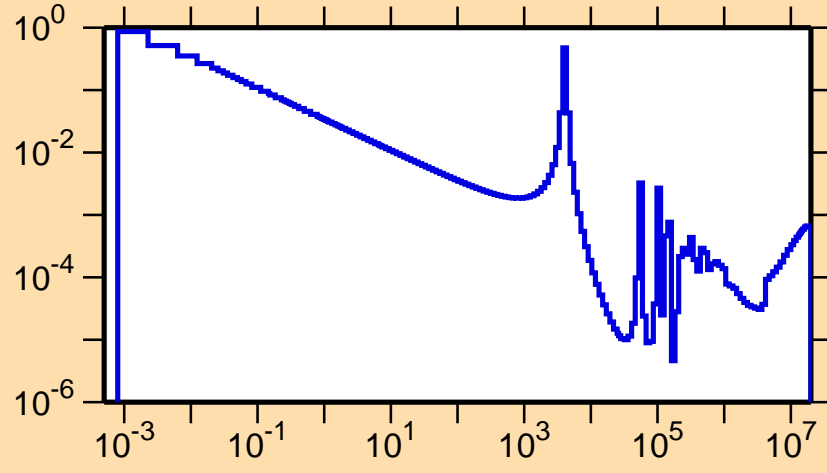
\sigma vs. E for ^{24}\text{Na}(n,\gamma)
