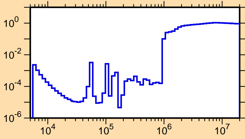
\sigma vs. E for ^{24}\text{Na}(n,\text{nonel.})
