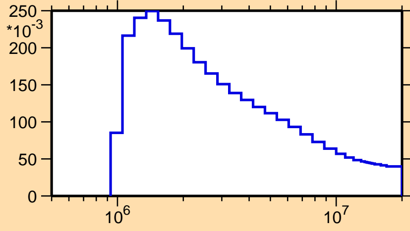
\sigma vs. E for ^{24}\text{Na}(n,n_2)
