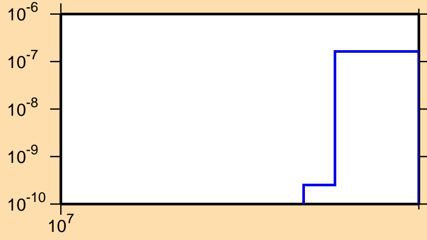
\sigma vs. E for ^{24}\text{Na}(n,p\alpha)
