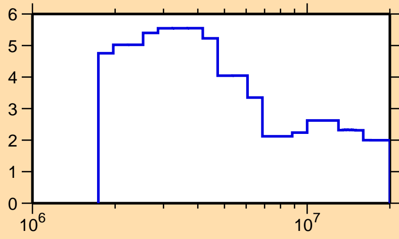
\Delta\sigma/\sigma vs. E for ^{24}\text{Na}(n,el.)
