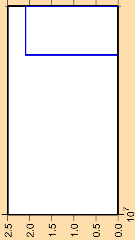
\Delta\sigma/\sigma vs. E for ^{24}\text{Na}(n,\text{He}3)
