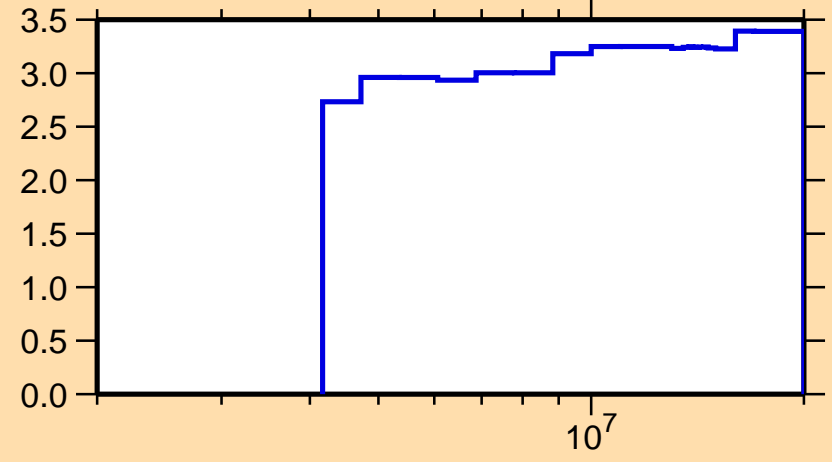
\Delta\sigma/\sigma vs. E for ^{24}\text{Na}(n,n\text{onel.})
