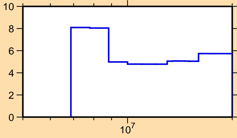
\Delta\sigma/\sigma vs. E for ^{24}\text{Na}(n,2n)
