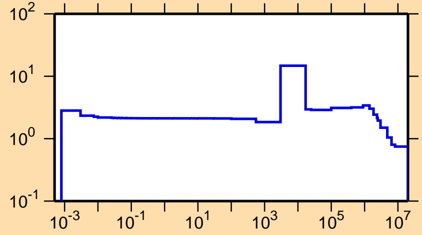
\sigma vs. E for ^{24}\text{Na}(n,\text{el.})
