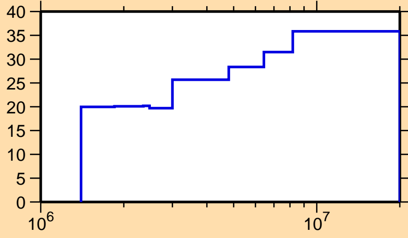
\Delta\sigma/\sigma vs. E for ^{24}\text{Na}(n,\gamma)
