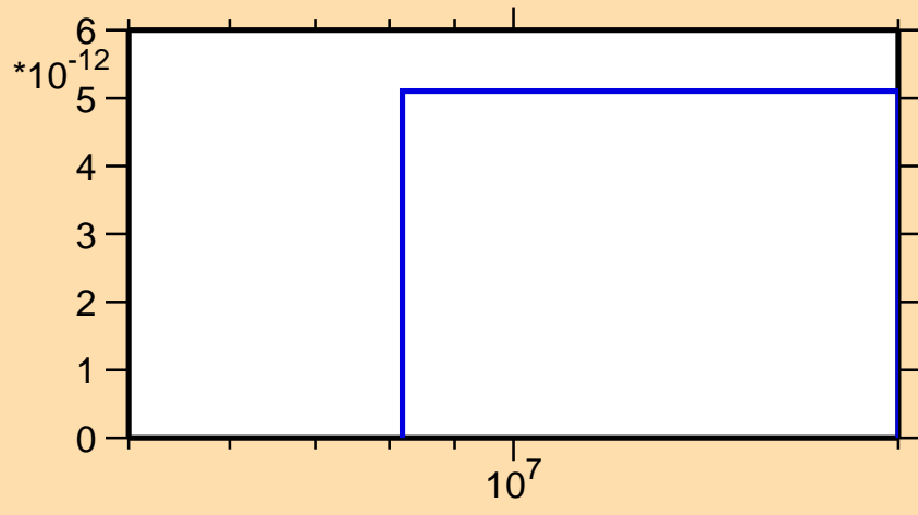
\sigma vs. E for ^{24}\text{Na}(n,2n\alpha)
