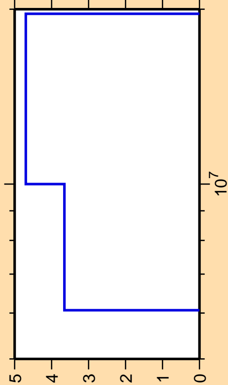
\Delta\sigma/\sigma vs. E for ^{25}\text{Na}(n,n_{\text{cont}})
