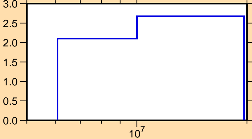
\Delta\sigma/\sigma vs. E for ^{25}\text{Na}(n,\text{el.})
