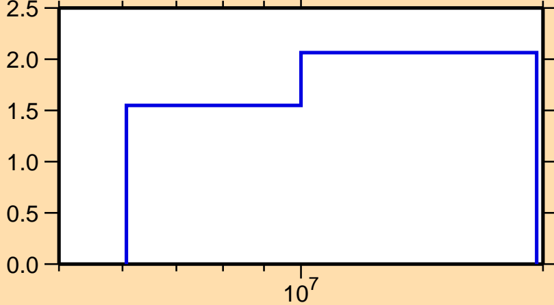
\Delta\sigma/\sigma vs. E for ^{25}\text{Na}(n,n\text{onel.})
