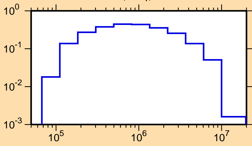
\sigma vs. E for ^{25}\text{Na}(n,n_1)
