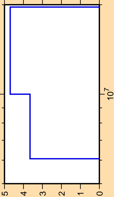
\Delta\sigma/\sigma vs. E for ^{25}\text{Na}(n,n\text{cont.})
