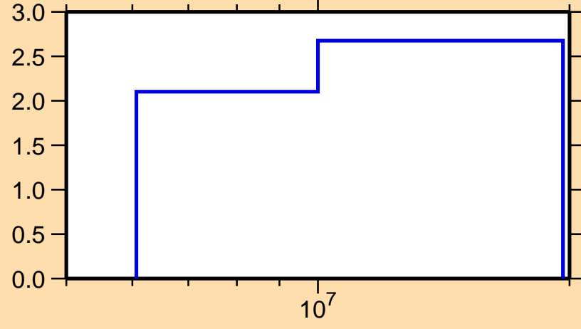
\Delta\sigma/\sigma vs. E for ^{25}\text{Na}(n,el.)
