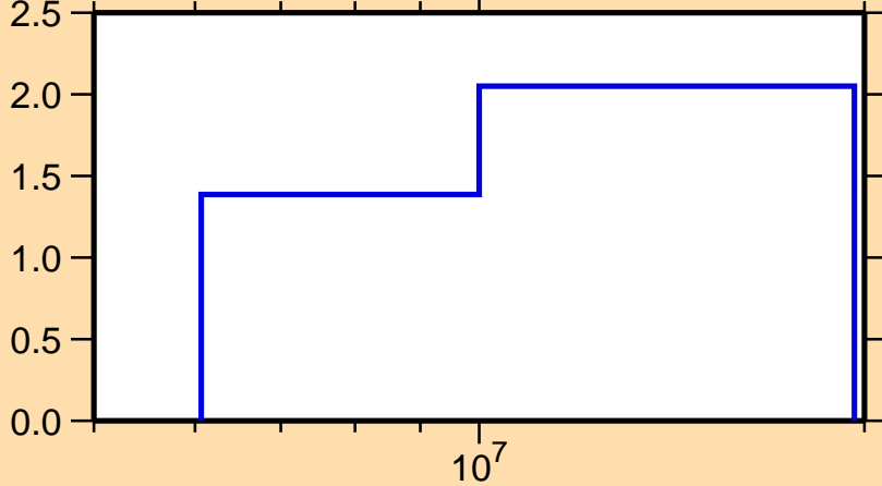
\Delta\sigma/\sigma vs. E for ^{25}\text{Na}(n,\text{inel.})
