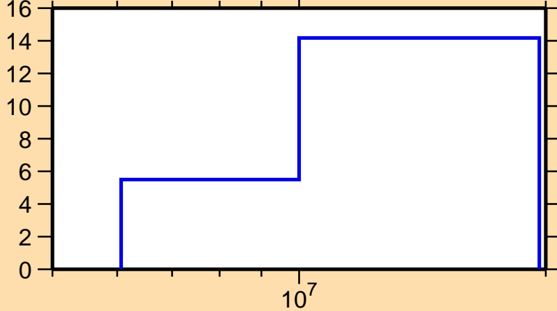
\Delta\sigma/\sigma vs. E for ^{25}\text{Na}(n,n_1)
