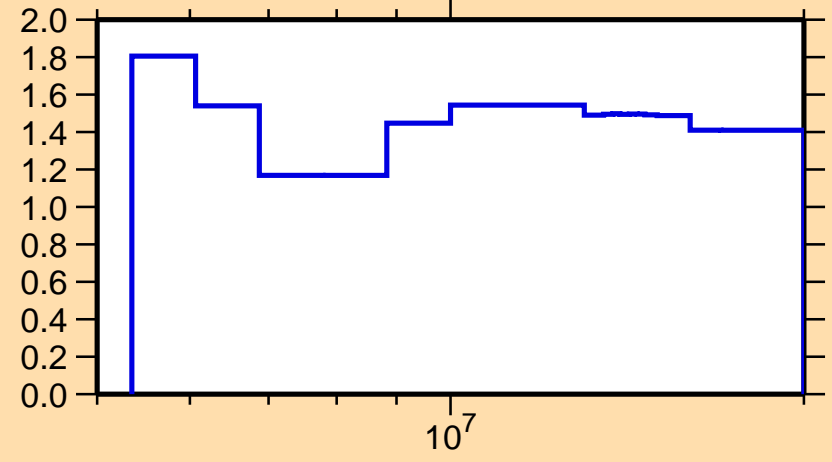
\Delta\sigma/\sigma vs. E for ^{26}\text{Na}(n,\text{tot.})
