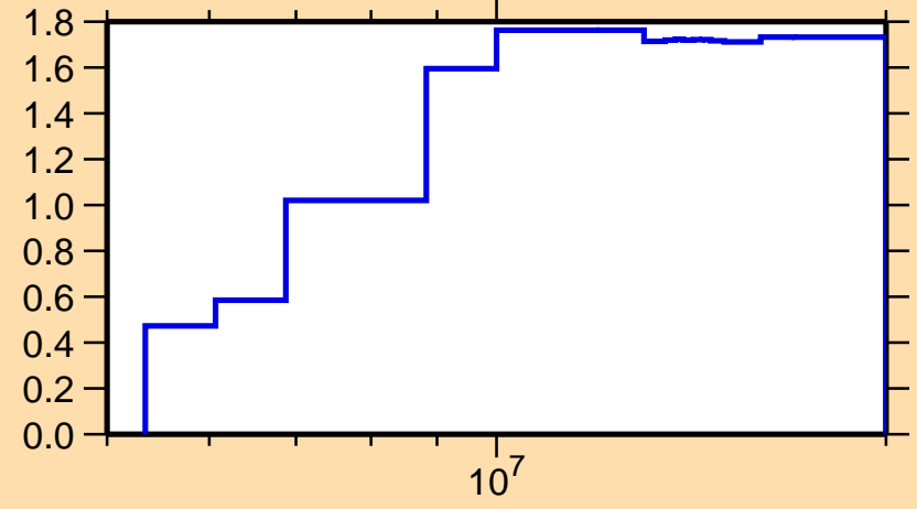
\Delta\sigma/\sigma vs. E for ^{26}\text{Na}(n,n\text{onel.})
