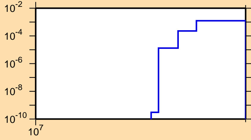
\sigma vs. E for ^{26}\text{Na}(n,\text{nd})
