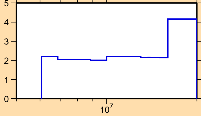
\Delta\sigma/\sigma vs. E for ^{26}\text{Na}(n,2n)
