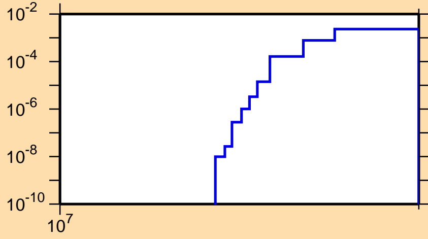
\sigma vs. E for ^{26}\text{Na}(n,n\alpha)
