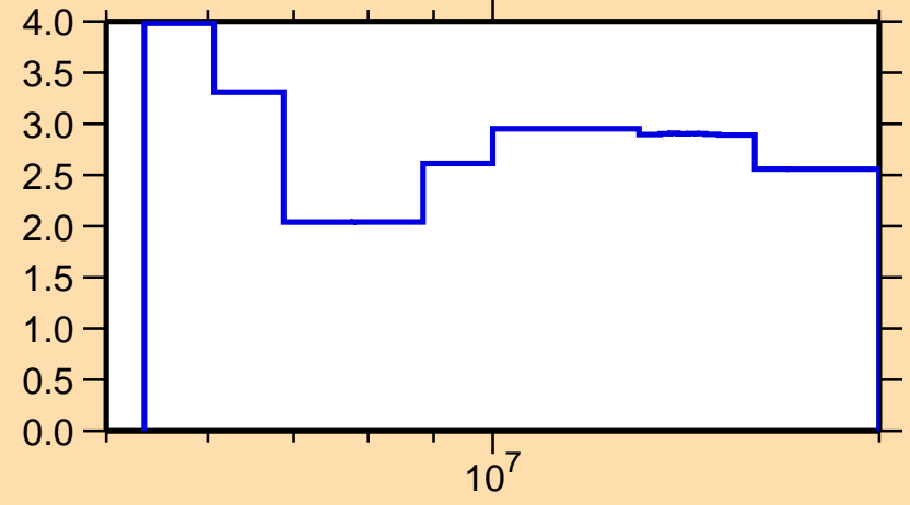
\Delta\sigma/\sigma vs. E for ^{26}\text{Na}(n,\text{el.})
