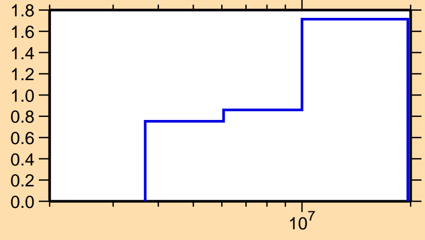
\Delta\sigma/\sigma vs. E for ^{26}\text{Na}(n,n\text{nonel.})
