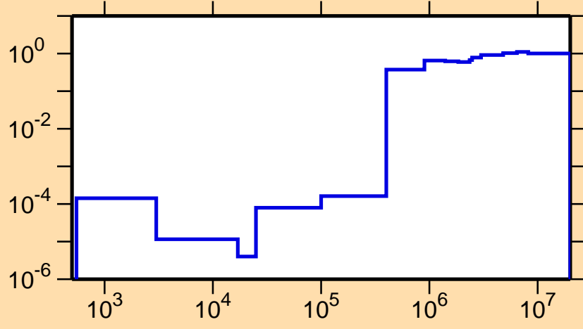
\sigma vs. E for ^{26}\text{Na}(n,\text{nonel.})
