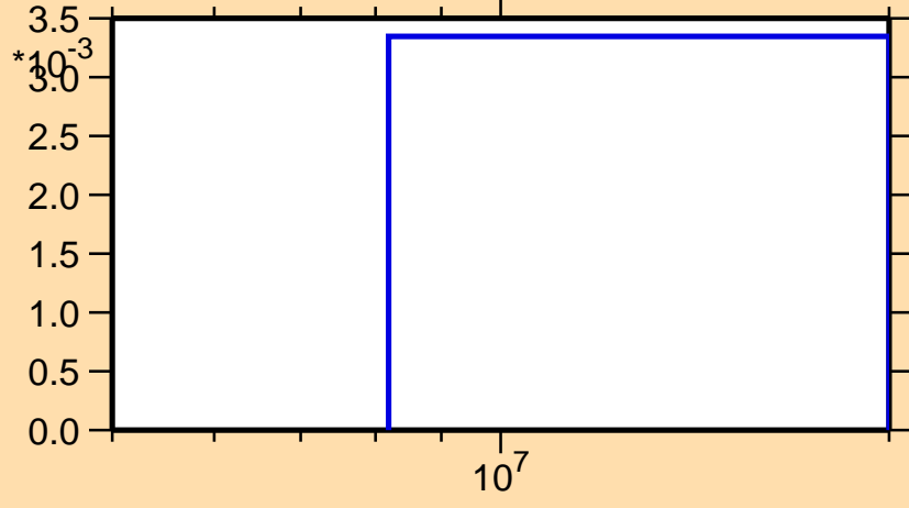
\sigma vs. E for ^{26}\text{Na}(n,d)
