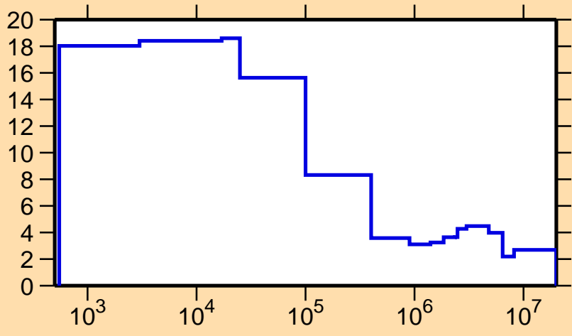
\Delta\sigma/\sigma vs. E for ^{26}\text{Na}(n,\text{el.})
