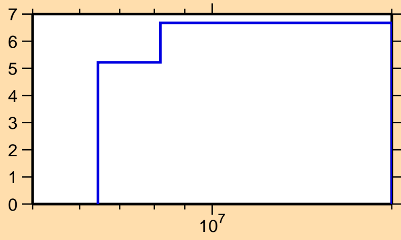
\Delta\sigma/\sigma vs. E for ^{26}\text{Na}(n,\text{inel.})
