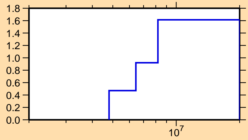
\Delta\sigma/\sigma vs. E for ^{26}\text{Na}(n,n\text{onel.})
