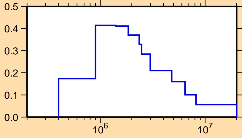
\sigma vs. E for ^{26}\text{Na}(n,n_3)
