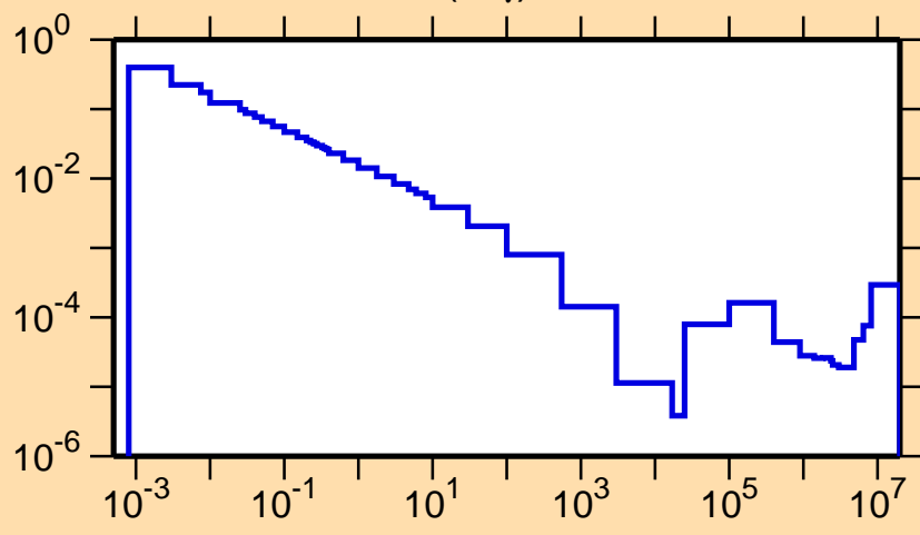
\sigma vs. E for ^{26}\text{Na}(n,\gamma)
