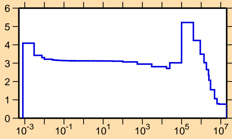
\sigma vs. E for ^{26}\text{Na}(n,\text{el.})
