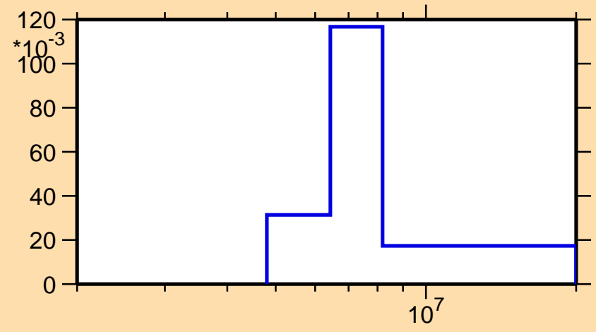
\sigma vs. E for ^{26}\text{Na}(n,n\text{cont.})
