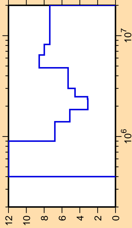
\Delta\sigma/\sigma vs. E for ^{26}\text{Na}(n,n_3)
