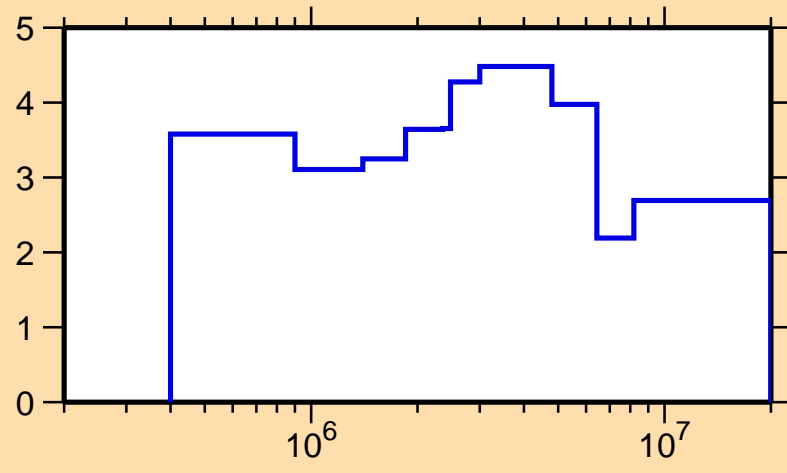
\Delta\sigma/\sigma vs. E for ^{26}\text{Na}(n,\text{el.})
