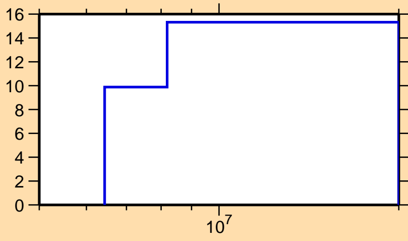
\Delta\sigma/\sigma vs. E for ^{26}\text{Na}(n,ncont.)
