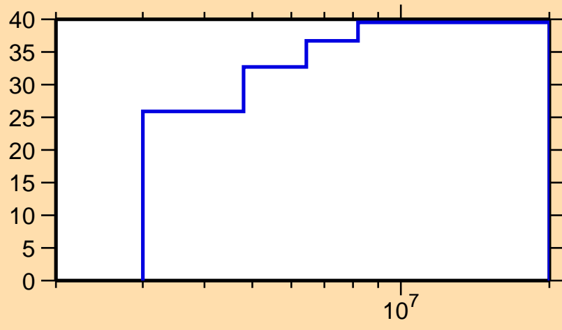
\Delta\sigma/\sigma vs. E for ^{26}\text{Na}(n,\gamma)
