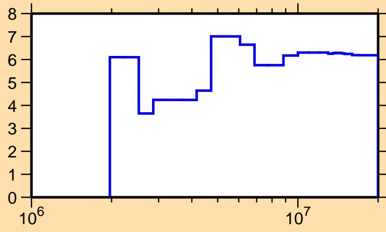
\Delta\sigma/\sigma vs. E for ^{83}\text{Nb}(n,n\text{nonel.})
