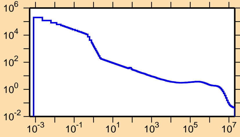
\sigma vs. E for ^{83}\text{Nb}(n,p)
