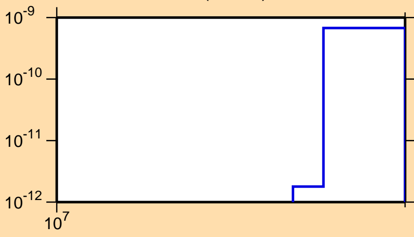
\sigma vs. E for ^{83}\text{Nb} (mt 34)
