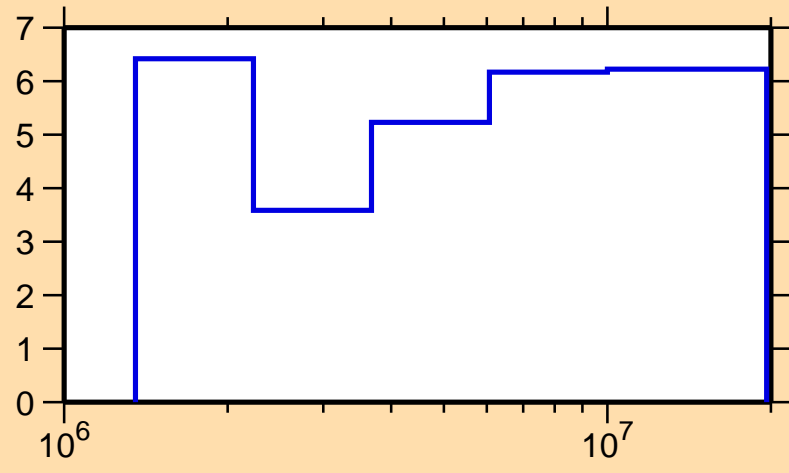
\Delta\sigma/\sigma vs. E for ^{83}\text{Nb}(n,\text{nonel.})
