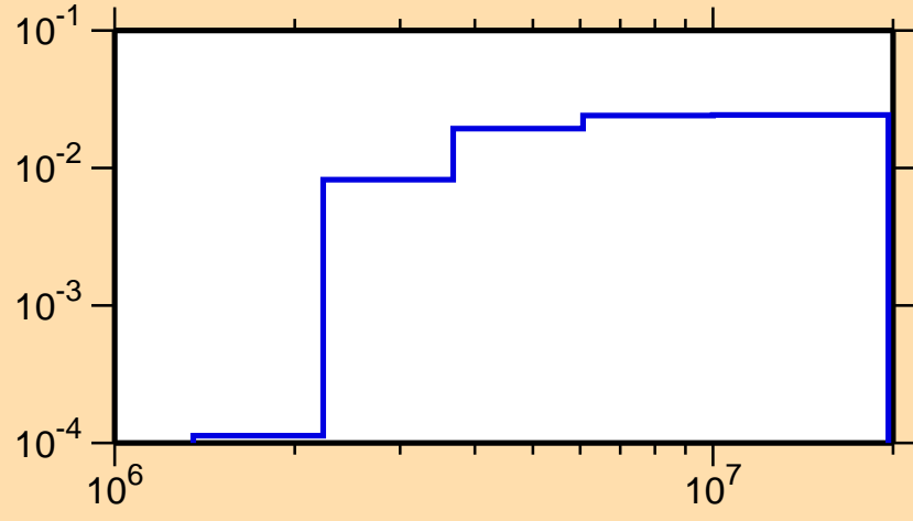
\sigma vs. E for ^{83}\text{Nb}(n,n\text{cont.})
