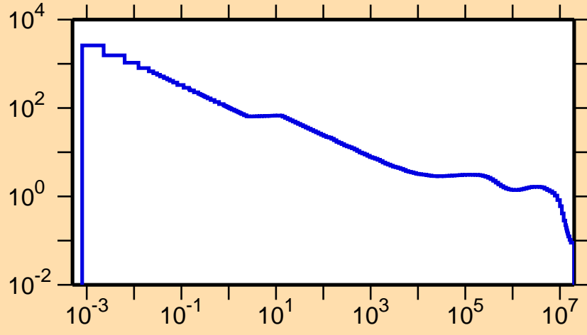
\sigma vs. E for ^{87}\text{Nb}(n,p)
