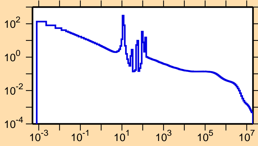
\sigma vs. E for ^{87}\text{Nb}(n,\gamma)
