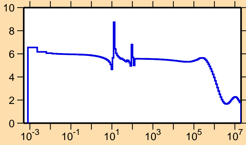
\sigma vs. E for ^{87}\text{Nb}(n,\text{el.})
