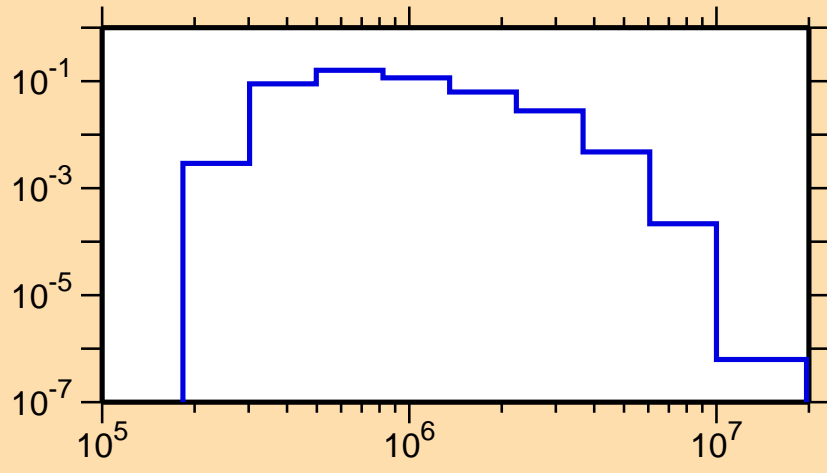
\sigma vs. E for ^{87}\text{Nb}(n,n_3)
