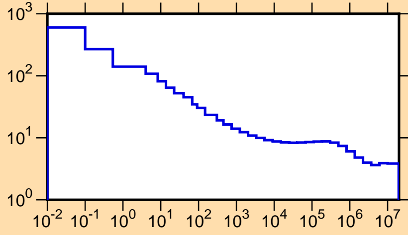
\sigma vs. E for ^{87}\text{Nb}(n,\text{tot.})
