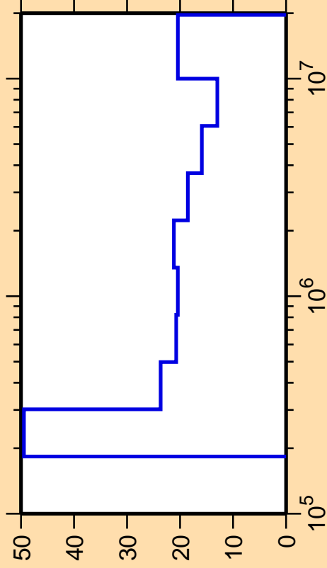
\Delta\sigma/\sigma vs. E for ^{87}\text{Nb}(n,n_3)
