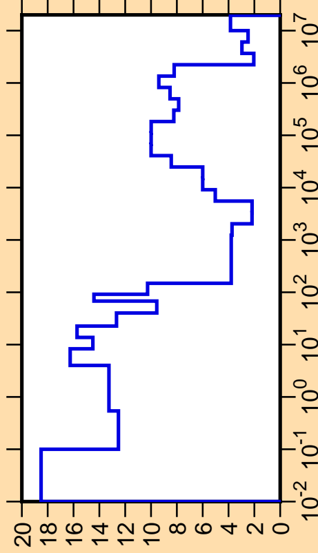
\Delta\sigma/\sigma vs. E for ^{87}\text{Nb}(n,\text{tot.})
