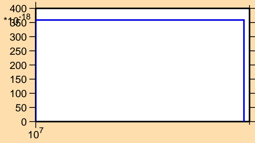
\sigma vs. E for ^{87}\text{Nb} (mt 34)
