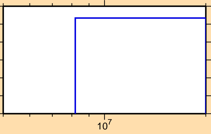
\sigma vs. E for ^{87}\text{Nb} (mt 34)
