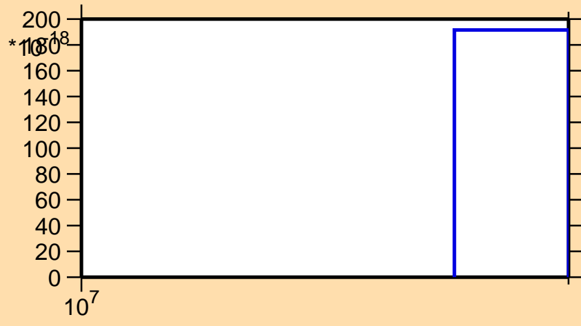
\sigma vs. E for ^{88}\text{Nb}(n,nt)
