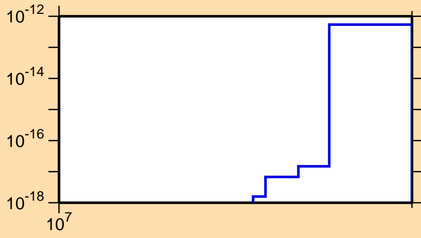
\sigma vs. E for ^{88}\text{Nb}(n,2n\alpha)
