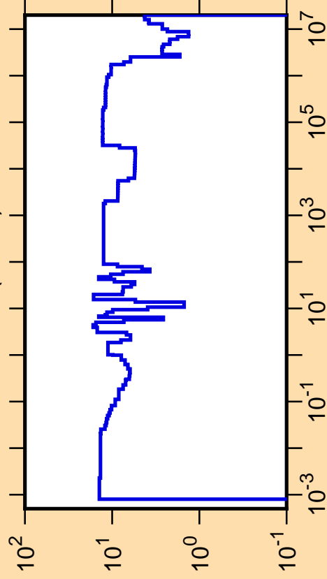
\Delta\sigma/\sigma vs. E for ^{88}\text{Nb}(n,\text{tot.})
