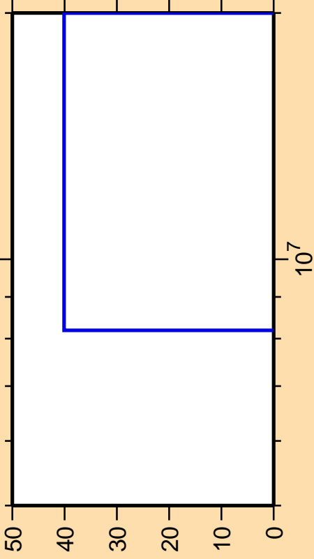
\Delta\sigma/\sigma vs. E for ^{88}\text{Nb}(\text{mt117})
