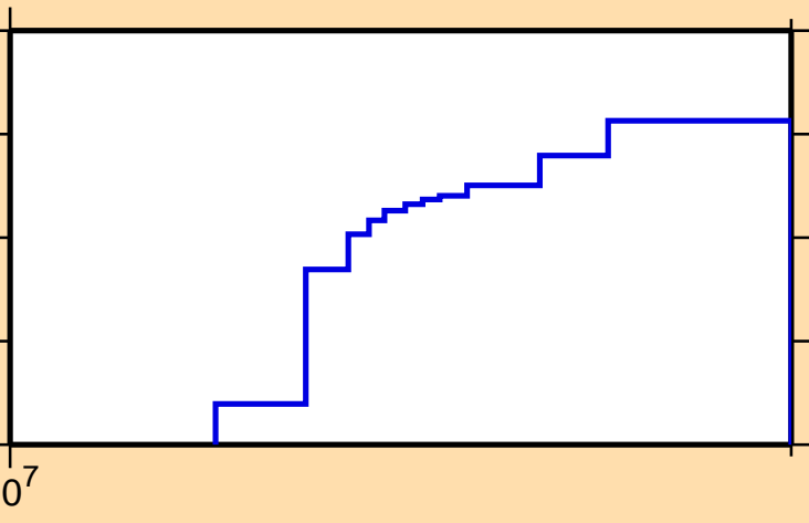
\sigma vs. E for ^{89}\text{Nb}(n,2n)
