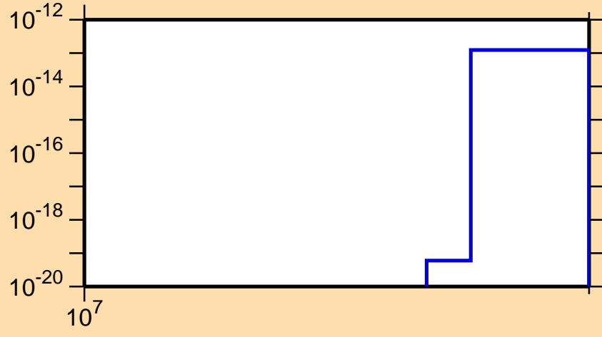
\sigma vs. E for ^{91}\text{Nb}(\text{mt } 45)
