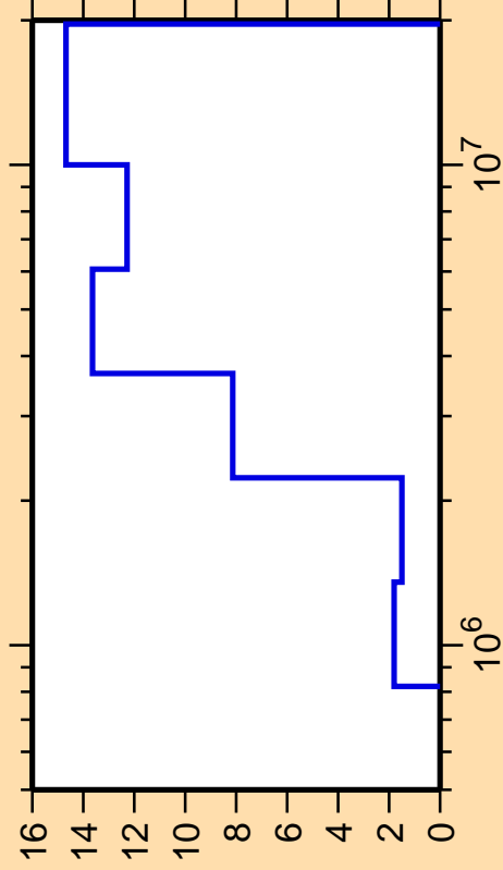
\Delta\sigma/\sigma vs. E for ^{91}\text{Nb}(n,n_2)
