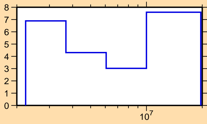
\Delta\sigma/\sigma vs. E for ^{91}\text{Nb}(n,n\text{cont.})
