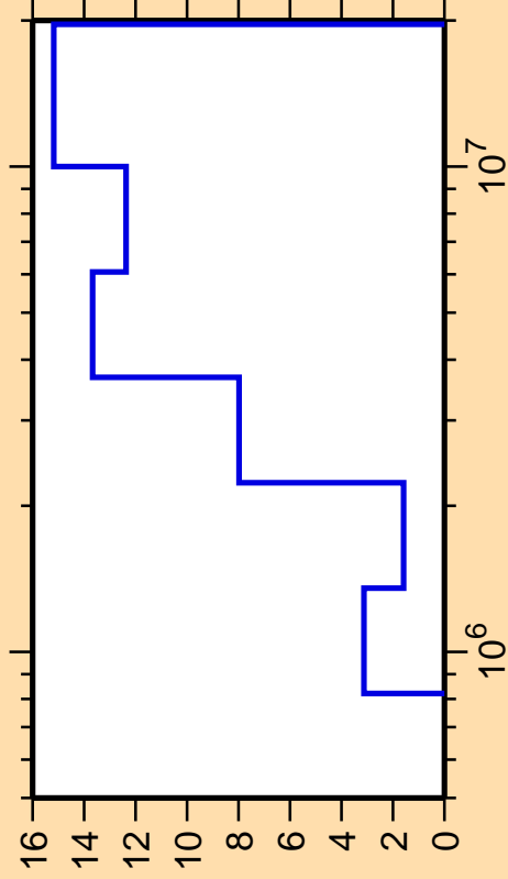
\Delta\sigma/\sigma vs. E for ^{91}\text{Nb}(n,n_4)
