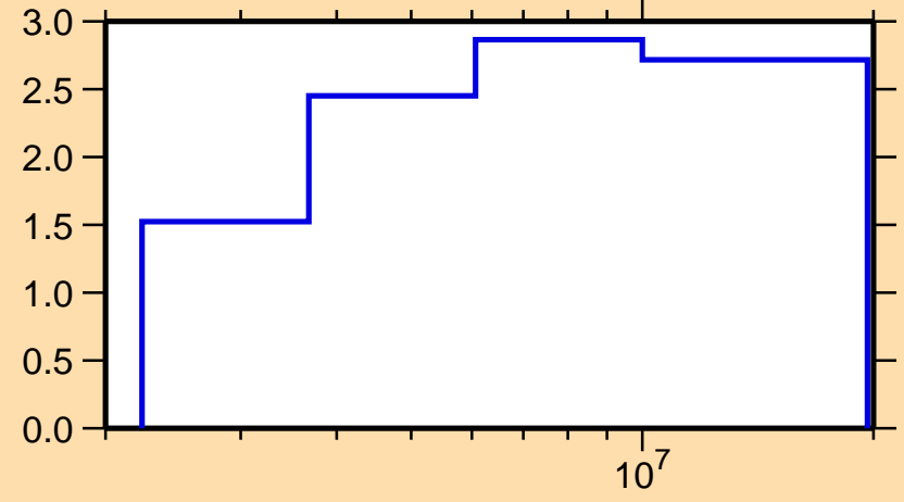
\Delta\sigma/\sigma vs. E for ^{91}\text{Nb}(n,n\text{nonel.})
