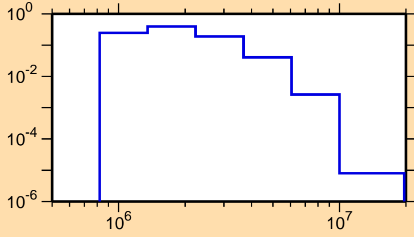
\sigma vs. E for ^{91}\text{Nb}(n,n_2)
