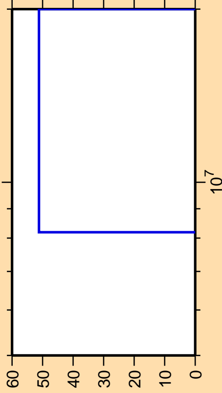
\Delta\sigma/\sigma vs. E for ^{91}\text{Nb}(n,p\alpha)
