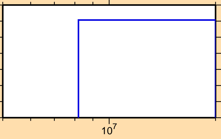
\sigma vs. E for ^{91}\text{Nb}(n,p\alpha)
