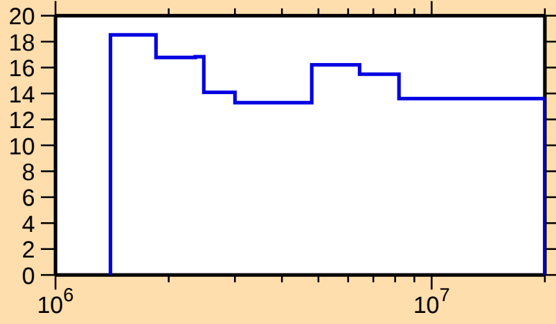
\Delta\sigma/\sigma vs. E for ^{92}\text{Nb}(n,n_1)
