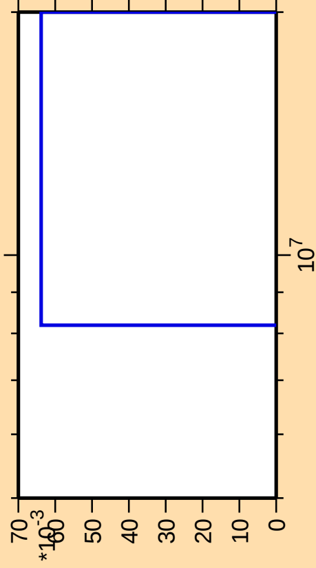
\Delta\sigma/\sigma vs. E for ^{92}\text{Nb}(\text{mt } 34)
