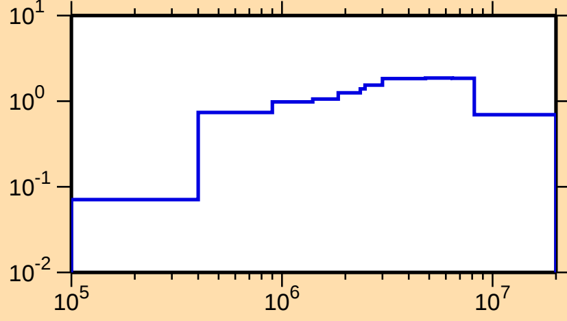
\sigma vs. E for ^{92}\text{Nb}(n,\text{inel.})
