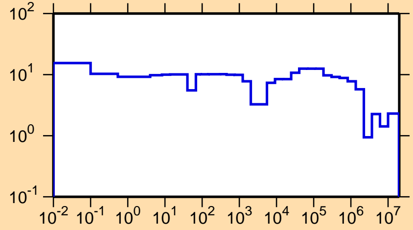
\Delta\sigma/\sigma vs. E for ^{93}\text{Nb}(n,\text{tot.})
