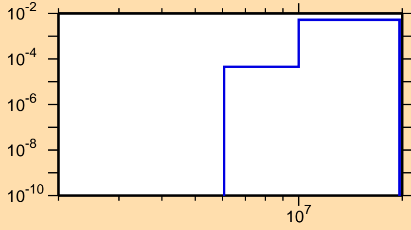
\sigma vs. E for ^{93}\text{Nb}(n,n\alpha)
