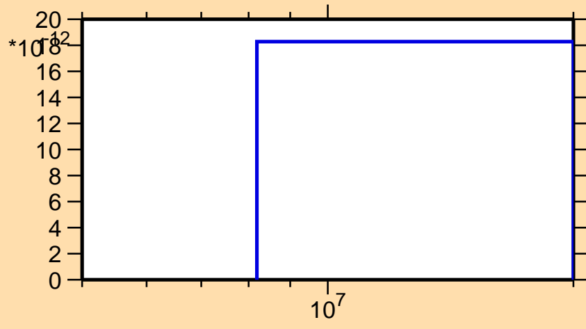
\sigma vs. E for ^{93}\text{Nb}(\text{mt } 45)
