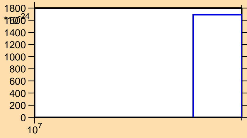
\sigma vs. E for ^{94}\text{Nb} (mt 11)
