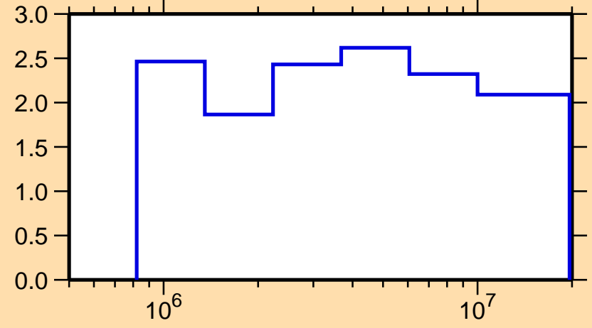
\Delta\sigma/\sigma vs. E for ^{94}\text{Nb}(n,n\text{nonel.})
