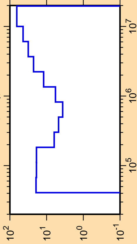
\Delta\sigma/\sigma vs. E for ^{94}\text{Nb}(n,n_1)
