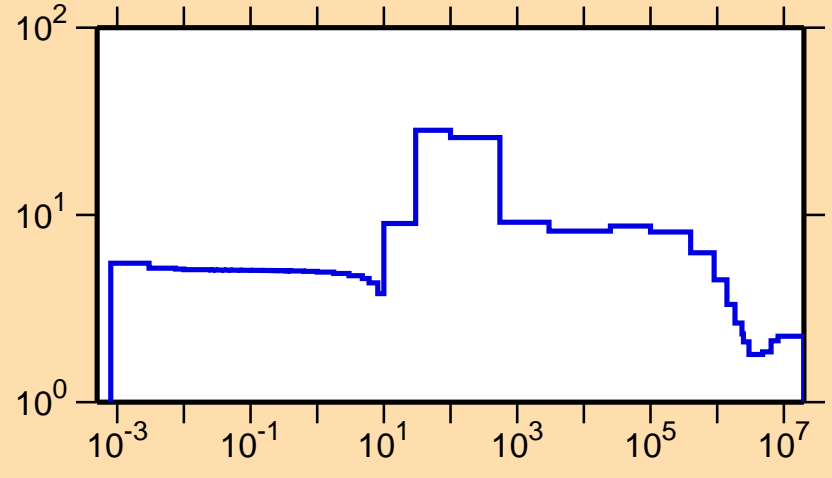
\sigma vs. E for ^{94}\text{Nb}(n,\text{el.})
