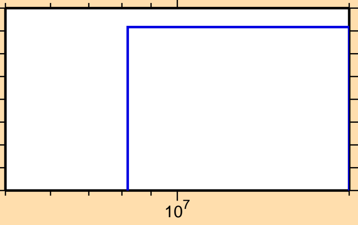
\sigma vs. E for ^{94}\text{Nb}(\text{mt } 45)
