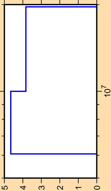
\Delta\sigma/\sigma vs. E for ^{94}\text{Nb}(n,2n)
