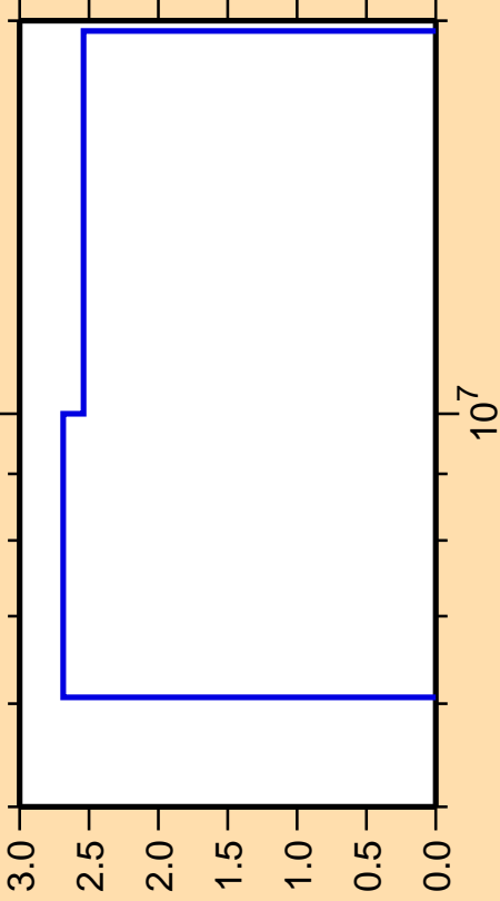
\Delta\sigma/\sigma vs. E for ^{95}\text{Nb}(n,2n)
