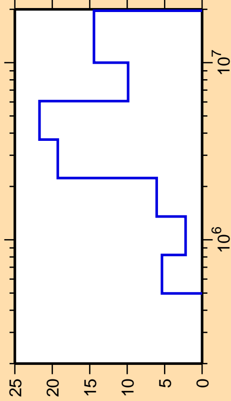
\Delta\sigma/\sigma vs. E for ^{95}\text{Nb}(n,n_4)
