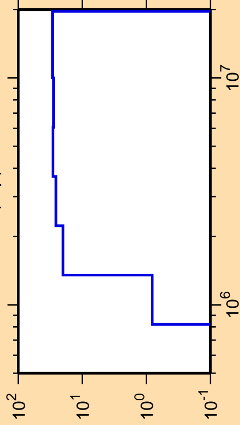
\Delta\sigma/\sigma vs. E for ^{95}\text{Nb}(n,p)
