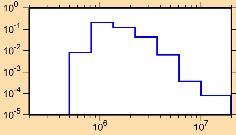
\sigma vs. E for ^{95}\text{Nb}(n,n_4)
