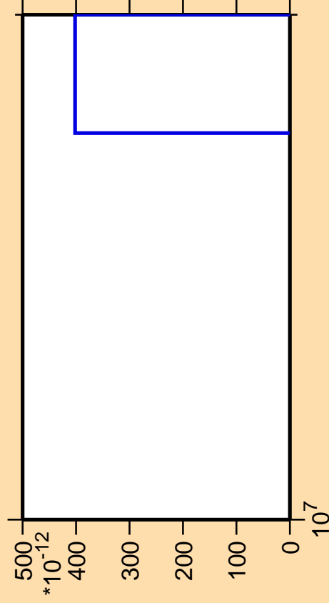
\Delta\sigma/\sigma vs. E for ^{96}\text{Nb} (mt 11)
