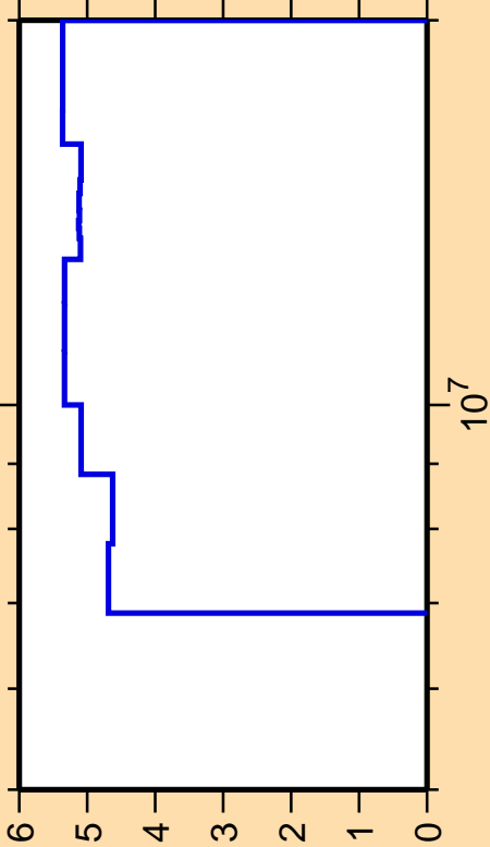
\Delta\sigma/\sigma vs. E for ^{96}\text{Nb}(n,2n)
