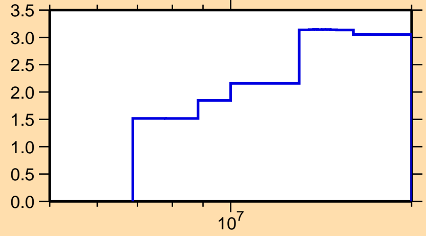
\Delta\sigma/\sigma vs. E for ^{96}\text{Nb}(n,\text{tot.})
