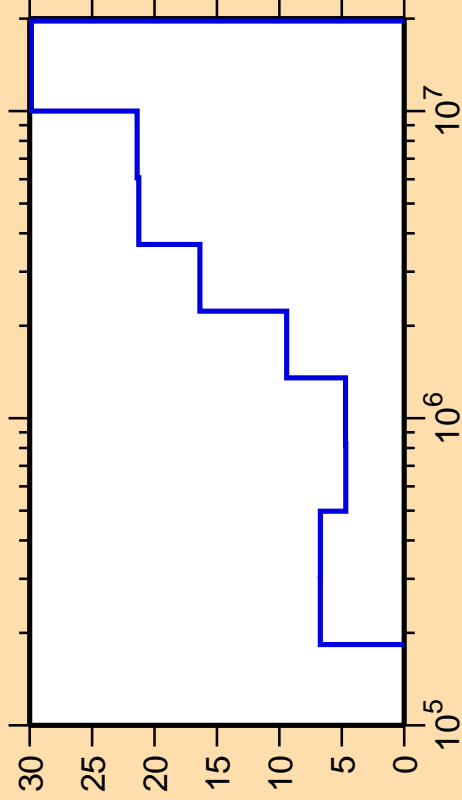
\Delta\sigma/\sigma vs. E for ^{96}\text{Nb}(n,n_3)
