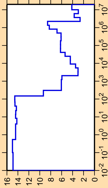
\Delta\sigma/\sigma vs. E for ^{96}\text{Nb}(n,\text{el.})
