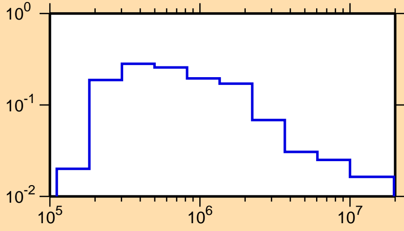
\sigma vs. E for ^{96}\text{Nb}(n,n_2)
