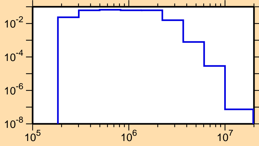
\sigma vs. E for ^{96}\text{Nb}(n,n_3)
