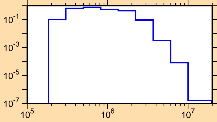
\sigma vs. E for ^{96}\text{Nb}(n,n_4)
