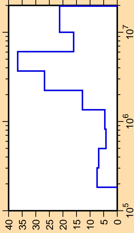
\Delta\sigma/\sigma vs. E for ^{96}\text{Nb}(n,n_4)
