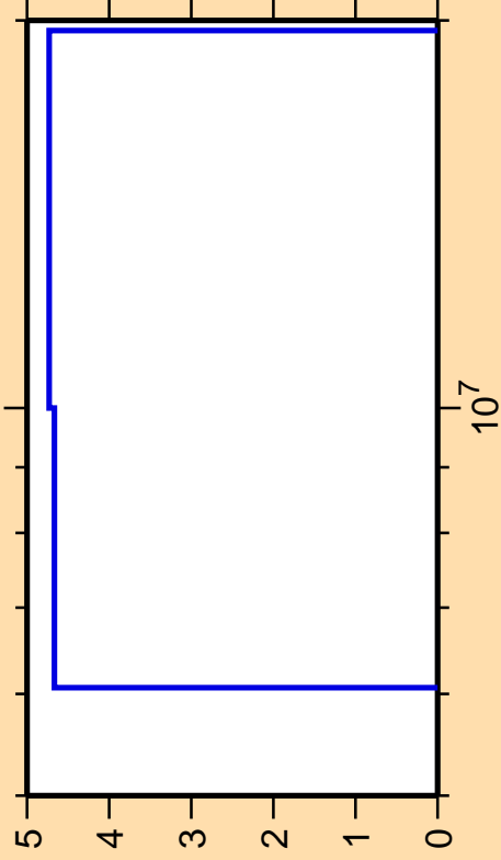
\Delta\sigma/\sigma vs. E for ^{96}\text{Nb}(n,2n)
