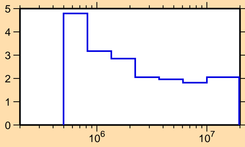
\Delta\sigma/\sigma vs. E for ^{96}\text{Nb}(n,\text{nonel.})
