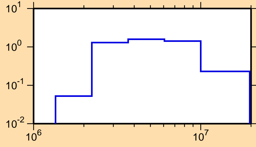
\sigma vs. E for ^{96}\text{Nb}(n,n\text{cont.})
