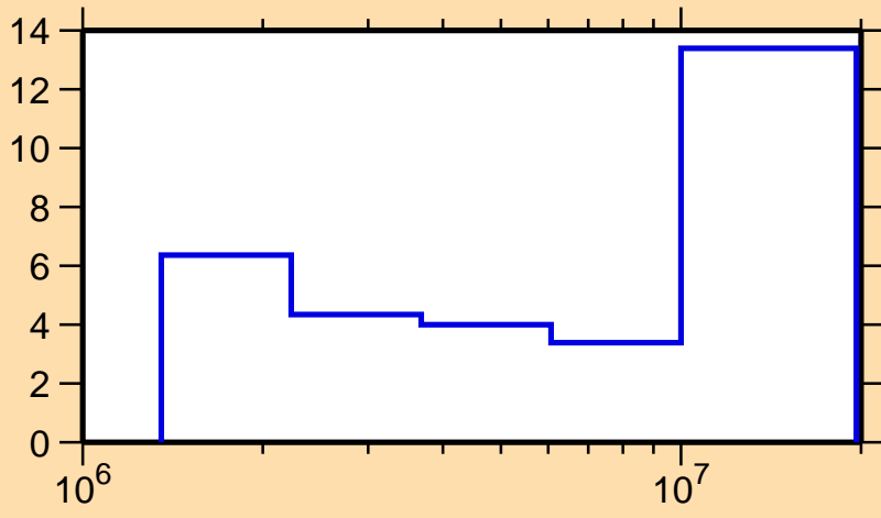
\Delta\sigma/\sigma vs. E for ^{96}\text{Nb}(n,n\text{cont.})
