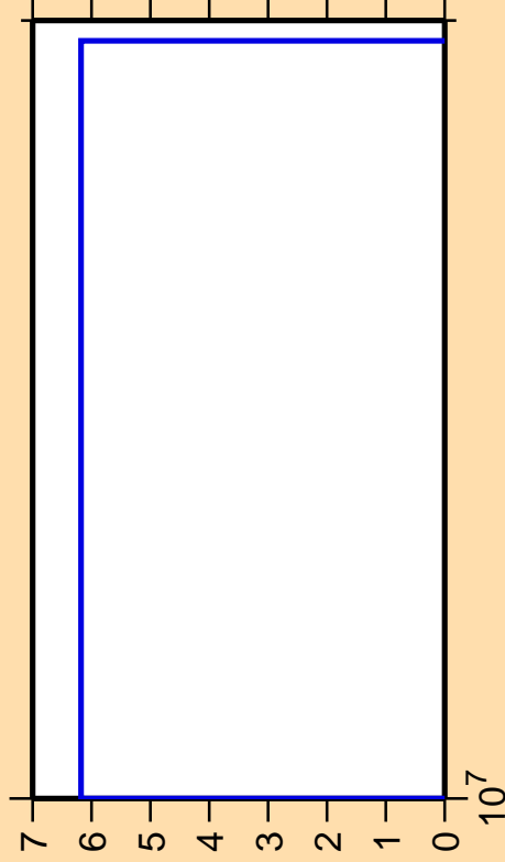
\Delta\sigma/\sigma vs. E for ^{96}\text{Nb}(n,p\alpha)
