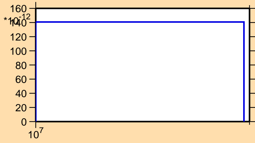
\sigma vs. E for ^{96}\text{Nb}(n,\text{He}3)
