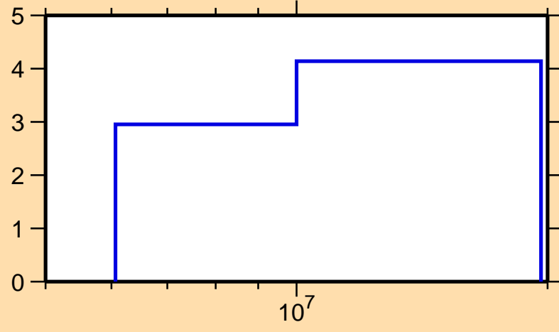
\Delta\sigma/\sigma vs. E for ^{96}\text{Nb}(n,\text{el.})
