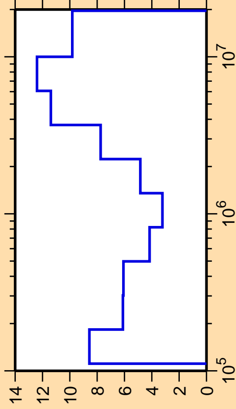
\Delta\sigma/\sigma vs. E for ^{96}\text{Nb}(n,n_2)
