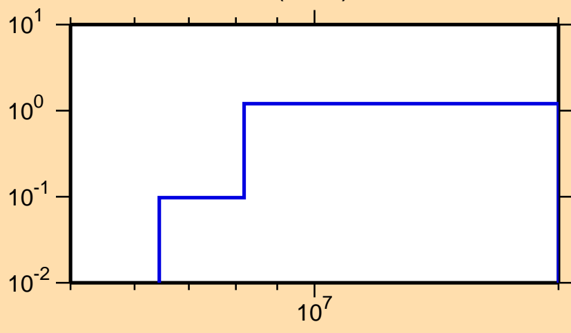
\sigma vs. E for ^{96}\text{Nb}(n,2n)
