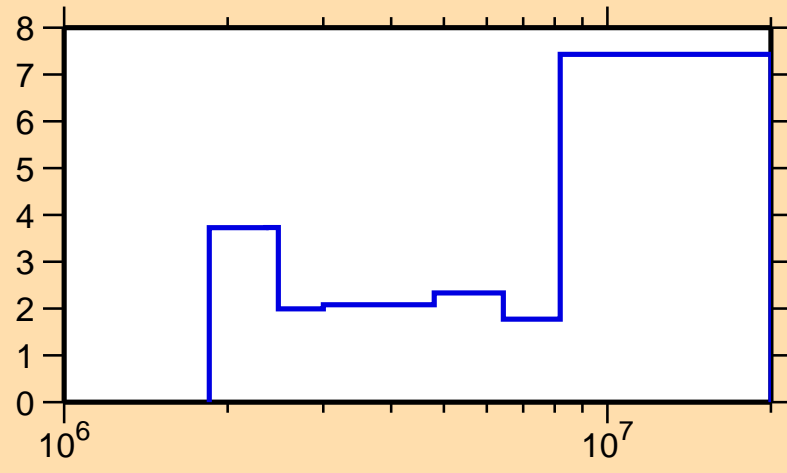
\Delta\sigma/\sigma vs. E for ^{96}\text{Nb}(n,\text{inel.})
