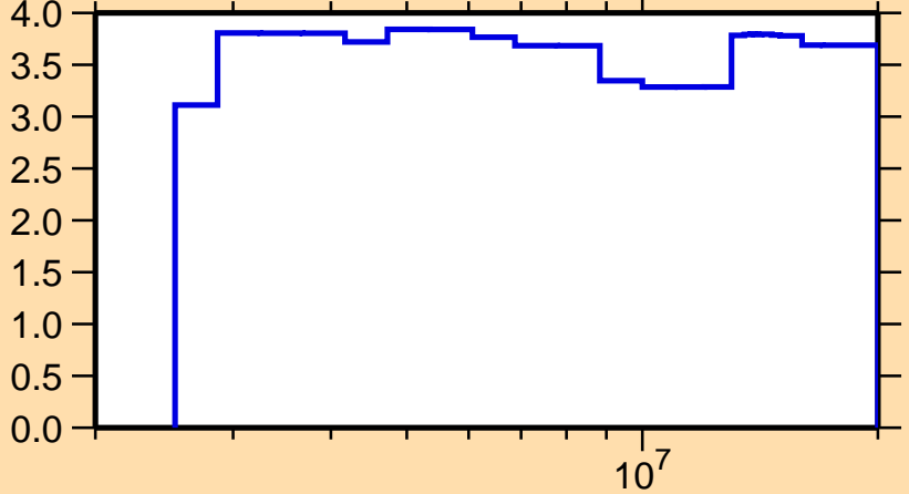
\Delta\sigma/\sigma vs. E for ^{97}\text{Nb}(n,n\text{onel.})
