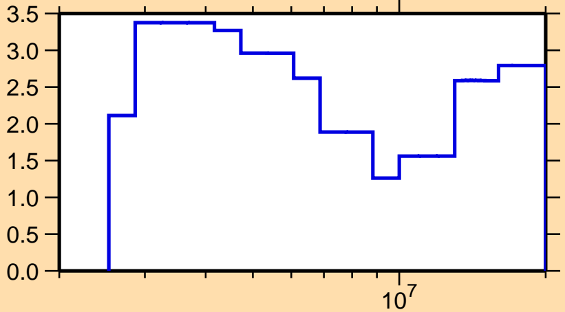
\Delta\sigma/\sigma vs. E for ^{97}\text{Nb}(n,\text{tot.})
