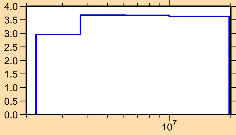
\Delta\sigma/\sigma vs. E for ^{97}\text{Nb}(n,n\text{onel.})
