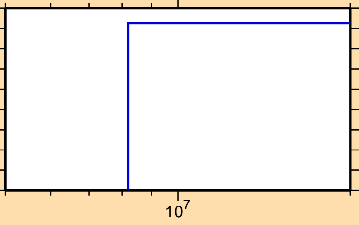
\sigma vs. E for ^{97}\text{Nb}(n,nt)
