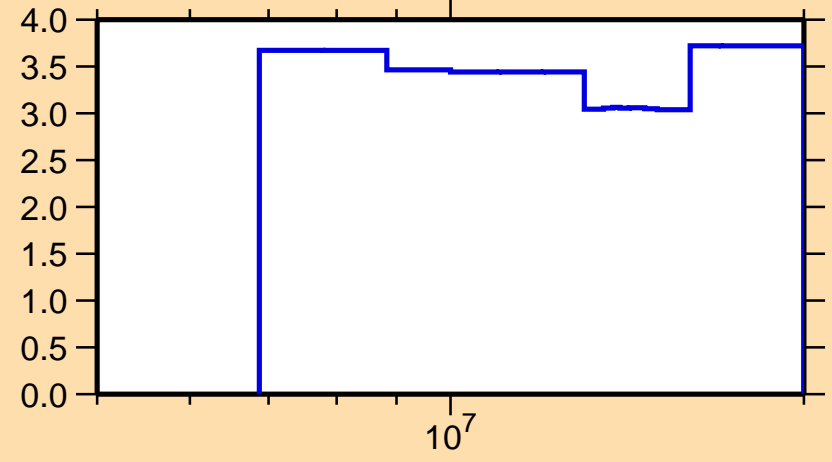
\Delta\sigma/\sigma vs. E for ^{97}\text{Nb}(n,\text{nonel.})
