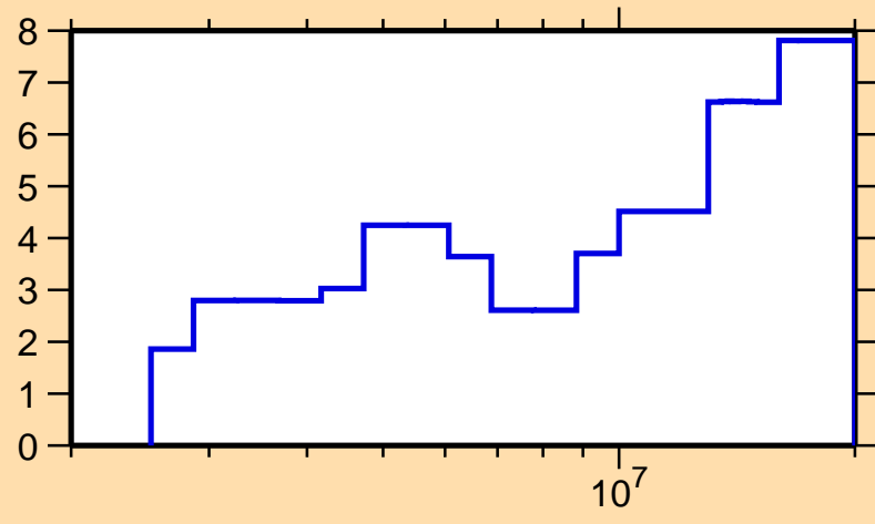
\Delta\sigma/\sigma vs. E for ^{98}\text{Nb}(n,el.)
