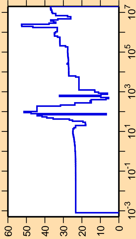
\Delta\sigma/\sigma vs. E for ^{98}\text{Nb}(n,\gamma)
