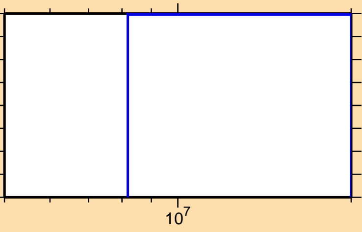
\sigma vs. E for ^{99}\text{Nb}(n,2np)
