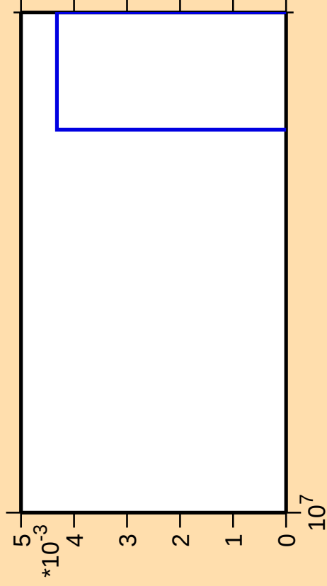
\Delta\sigma/\sigma vs. E for ^{100}\text{Nb}(\text{mt } 11)
