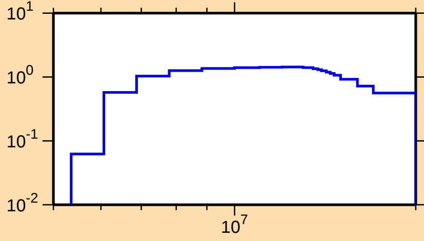
\sigma vs. E for ^{100}\text{Nb}(n,2n)
