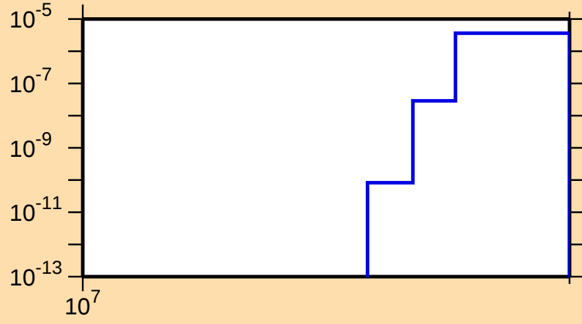
\sigma vs. E for ^{100}\text{Nb}(n,2np)
