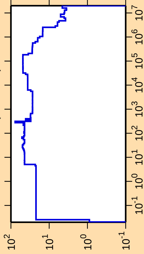
\Delta\sigma/\sigma vs. E for ^{100}\text{Nb}(n,\text{nonel.})
