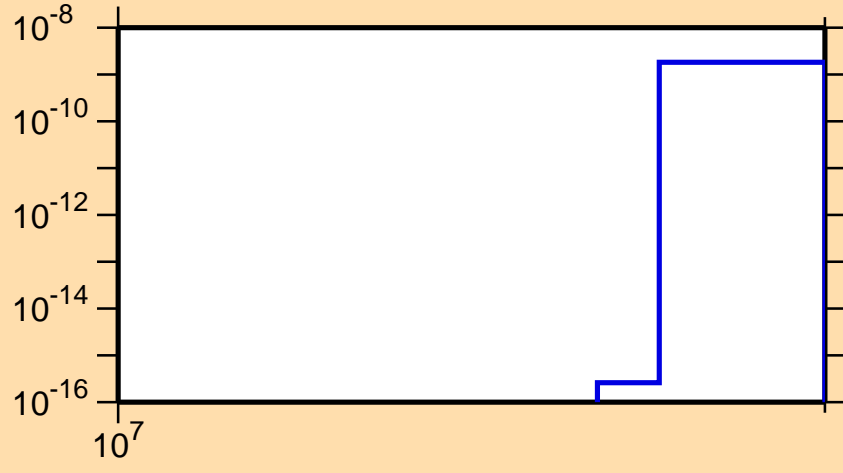
\sigma vs. E for ^{101}\text{Nb}(n,2np)
