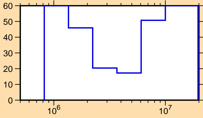
\Delta\sigma/\sigma vs. E for ^{101}\text{Nb}(n,n\text{cont.})
