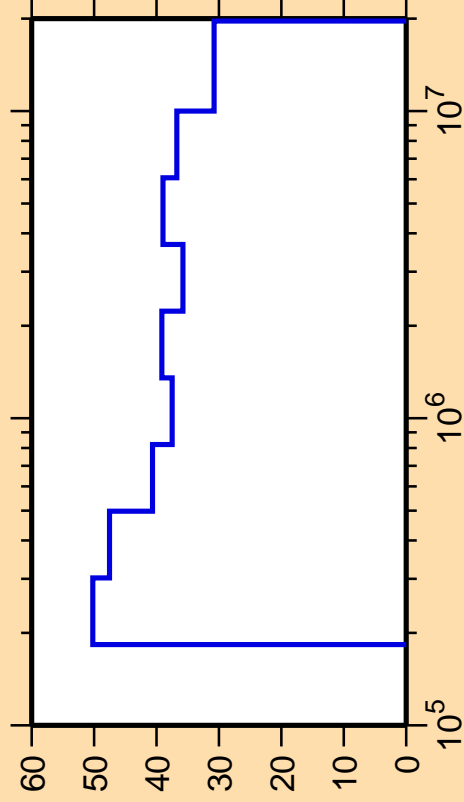
\Delta\sigma/\sigma vs. E for ^{101}\text{Nb}(n,n_4)
