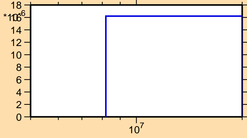
\sigma vs. E for ^{101}\text{Nb}(n,t)
