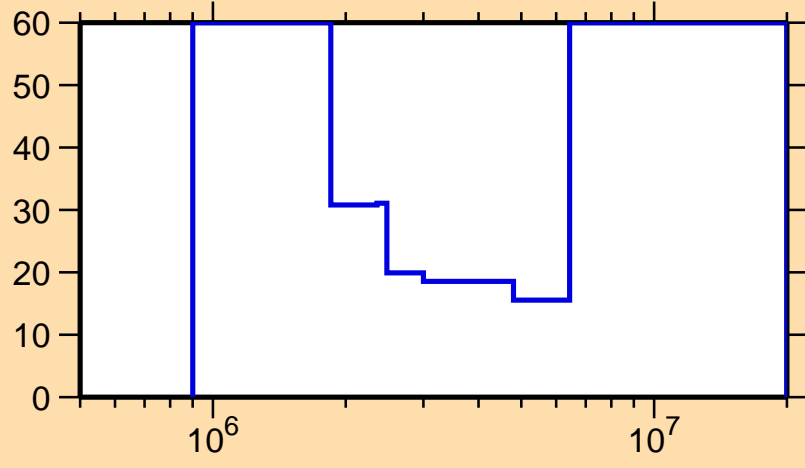
\Delta\sigma/\sigma vs. E for ^{101}\text{Nb}(n,n\text{cont.})
