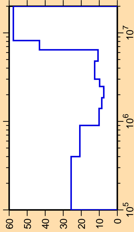
\Delta\sigma/\sigma vs. E for ^{101}\text{Nb}(n,\text{inel.})
