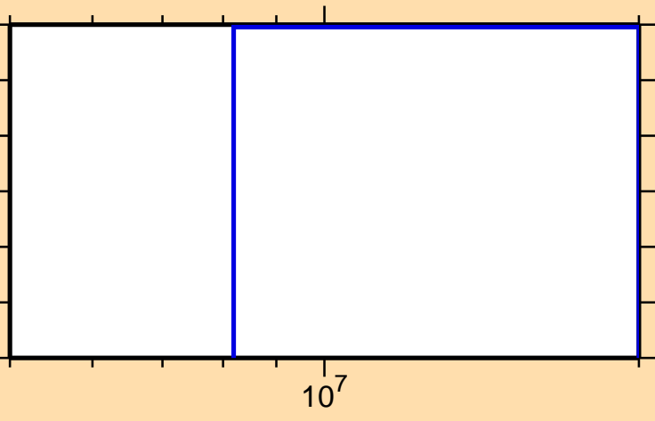
\sigma vs. E for ^{101}\text{Nb}(n,n\alpha)
