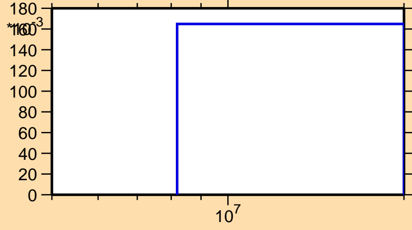
\sigma vs. E for ^{101}\text{Nb}(n,3n)
