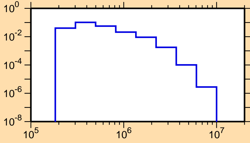
\sigma vs. E for ^{102}\text{Nb}(n,n_1)
