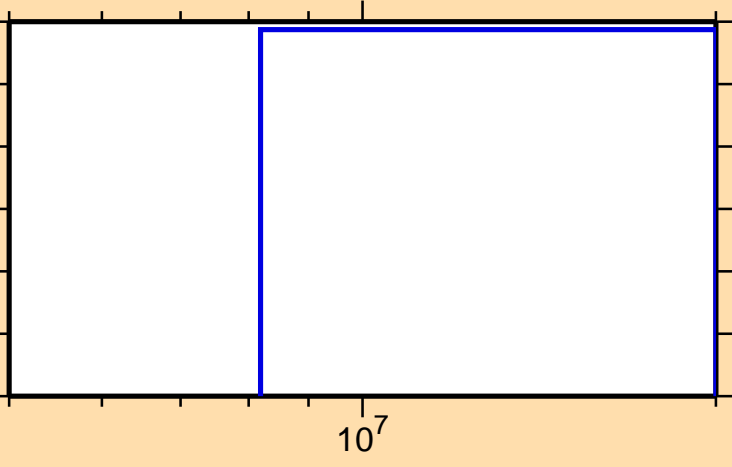
\sigma vs. E for ^{102}\text{Nb}(n,np)
