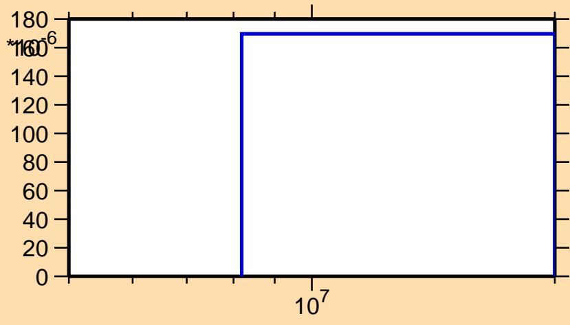
\sigma vs. E for ^{102}\text{Nb}(n,d)
