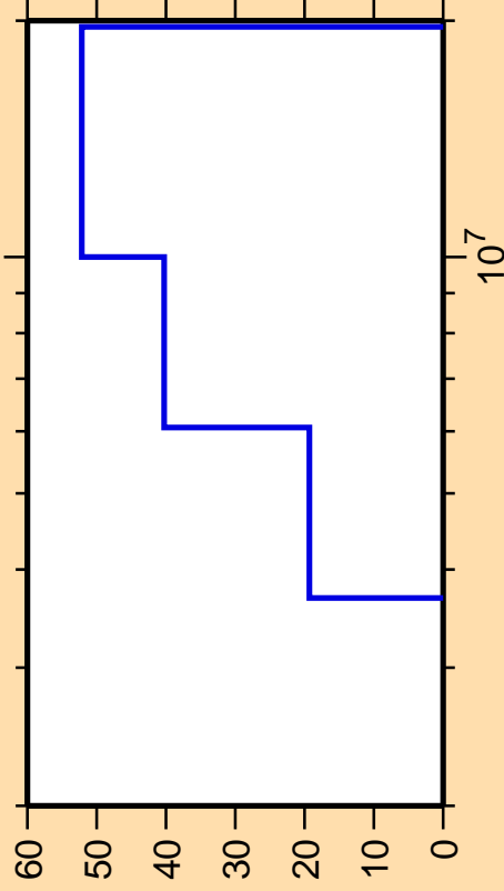
\Delta\sigma/\sigma vs. E for ^{102}\text{Nb}(n,n\text{cont.})
