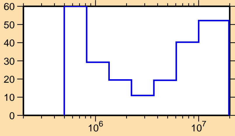
\Delta\sigma/\sigma vs. E for ^{102}\text{Nb}(n,n\text{cont.})
