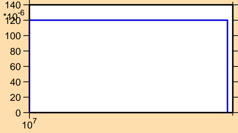
\sigma vs. E for ^{102}\text{Nb}(n,np)
