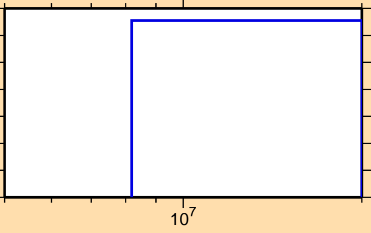
\sigma vs. E for ^{102}\text{Nb}(n,t)
