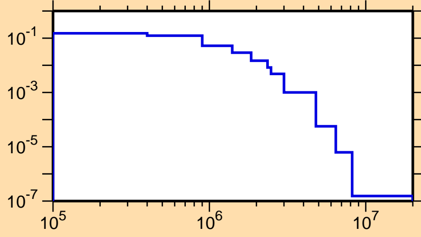
\sigma vs. E for ^{102}\text{Nb}(n,n_2)
