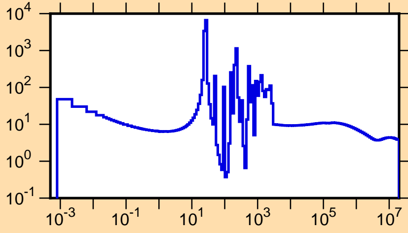
\sigma vs. E for ^{103}\text{Nb}(n,\text{tot.})
